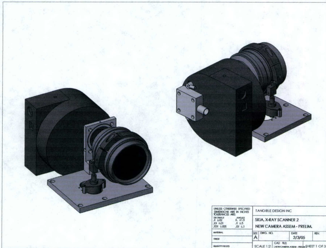
Figure 2 The X-ray lens and optical camera assembly inside the shielded box of figure 1.
