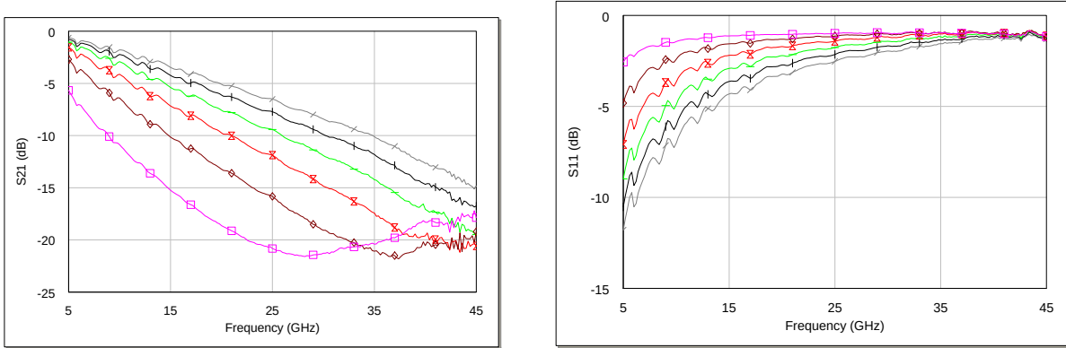
Figure 5. The experimental swept frequency response for a 7.5 x 7.5 \mu\text{m}^2 varactor shunt switch for 0V (pink) to 10 V (grey) with a step size of 2 V.
