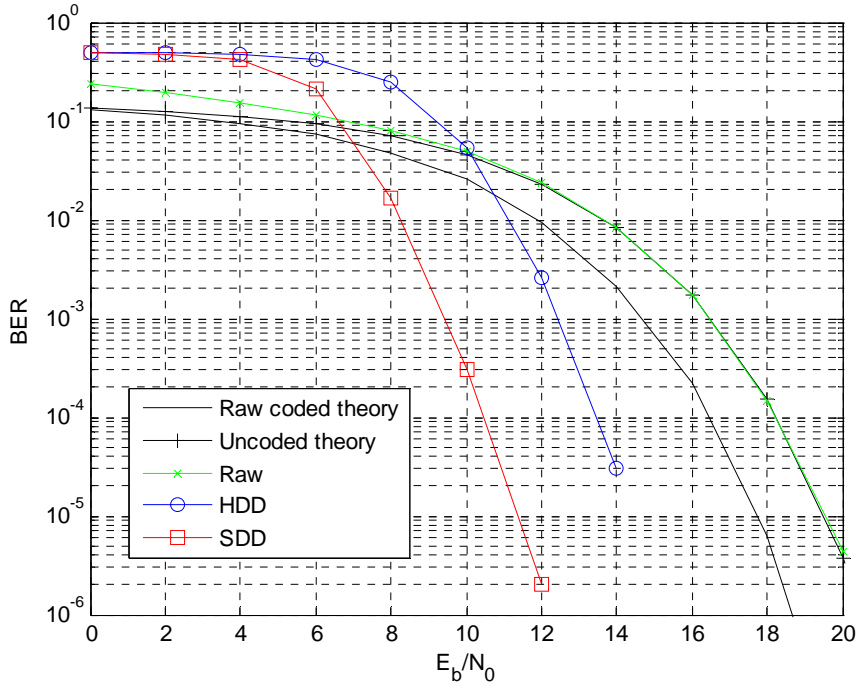
Figure 37. BER of Rate 2/3 64-QAM
