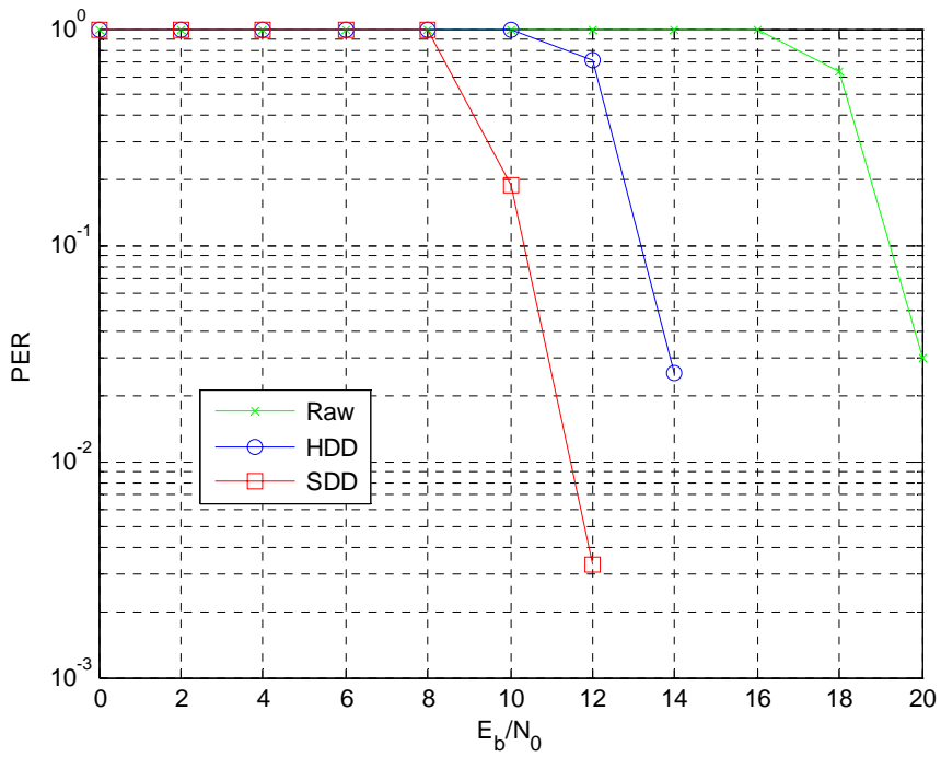
Figure 38. PER of Rate 2/3 64-QAM
