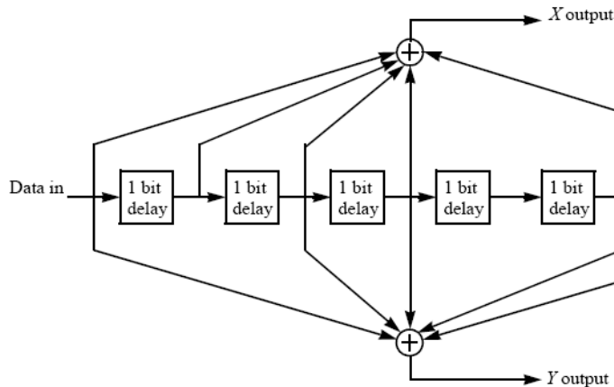
Figure 28. Binary rate 1/2 Convolutional Encoder (From Ref. [1].)
