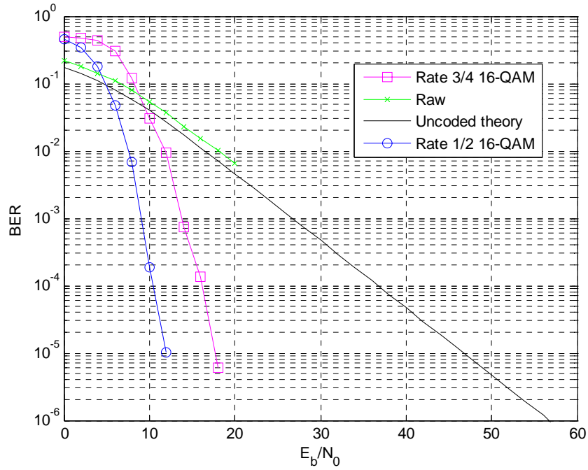
Figure 45. 16-QAM in 200-ns RMS Delay Spread Rayleigh-Fading Channel
