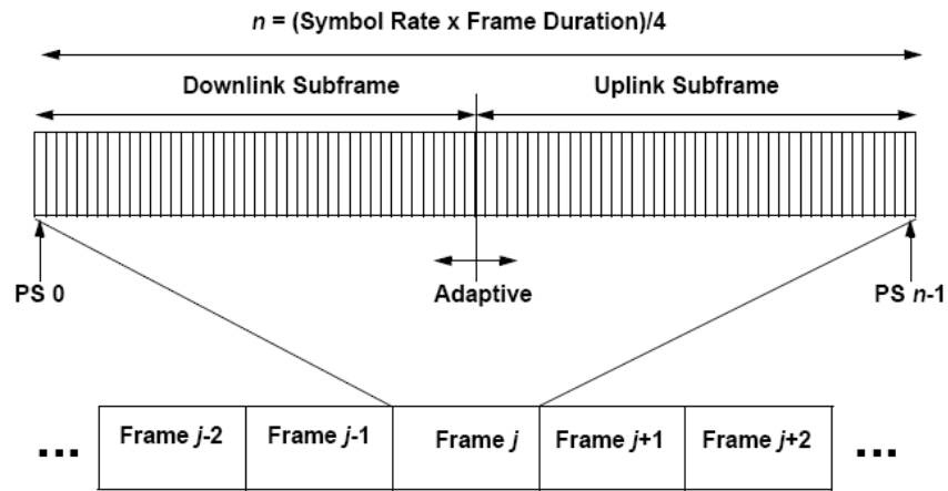
Figure 2. Example of TDD (From Ref. [1].)
