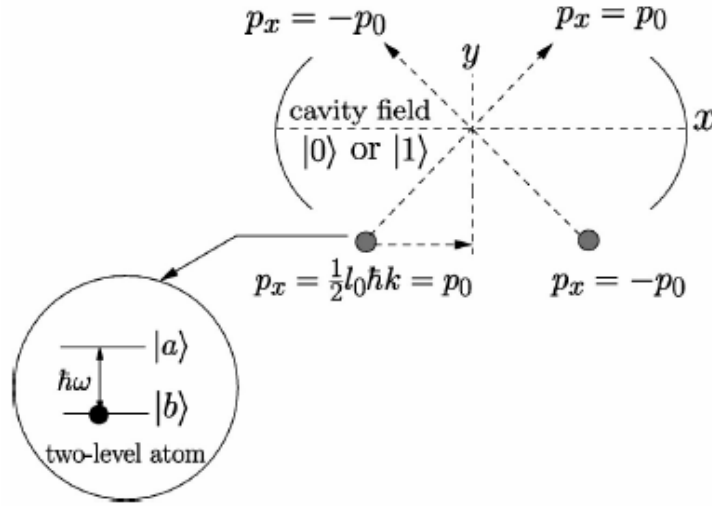
Figure 6: Atomic momentum state teleportation
