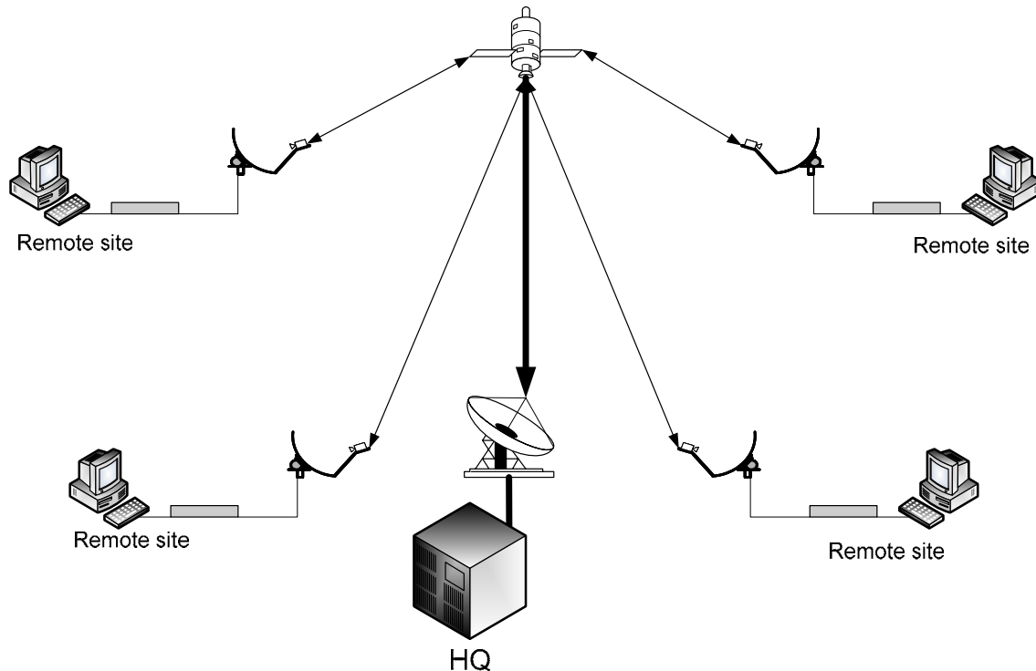
Figure 8. Star Topology
