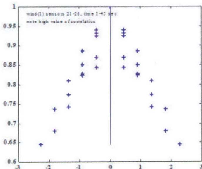
Figure 14: Pressure Field Correlation Measurements. This figure, from [20] shows how the pressure field correlation depends upon the separation (in meters) between two sensors. In order for spatial averaging to be effective under these conditions, the system must average over length scales of many meters.
