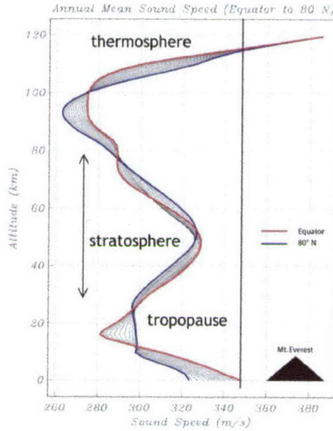
Figure 8: Typical sound speed vs. elevation, from Hedlin [34]
