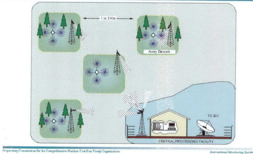
Figure 16: Infrasound monitoring station layout, from [22]
