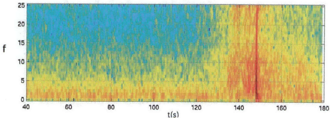
Figure 7: Acoustic spectrum of a Scud missile launch, measured at a range of 27 km. The launch took place at a time a bit less than 150 sec on this plot. Source: S. Tenney, ARL.
