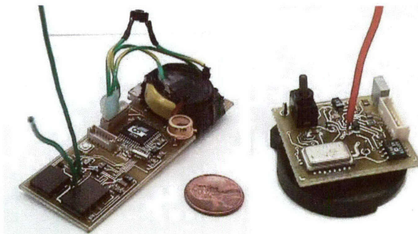
Figure 19: Commercial off the shelf wireless nodes from the Smart Dust group
