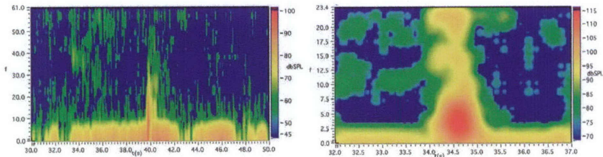
Figure 6: Left panel: Acoustic spectrum as a function of time (in seconds) of an artillery launch seen from 8.6 km. The launch took place at a time of about 40 sec on this plot. Right panel: Acoustic spectrum of an MLRS missile launch seen from 9 km. This launch (or launches; the documentation was unclear on this) took place at about 34.6 sec. Source: S. Tenney, ARL.
