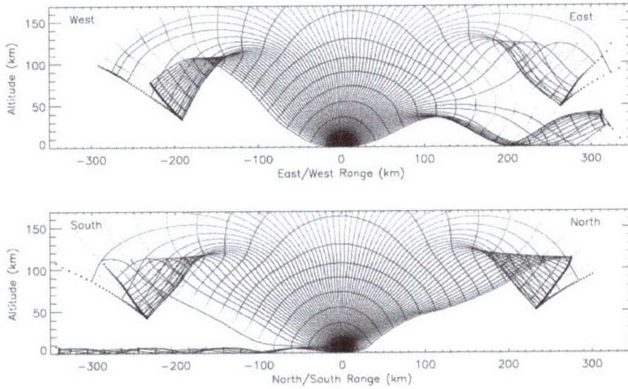
Figure 10: Model calculation of sonic propagation. Note the low-elevation duct in the lower panel, due to ambient wind. From [1]
