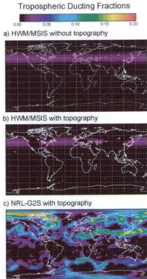
Figure 12: Combining low elevation meteorology with upper atmosphere models. This figure is taken from reference [1], and shows (in the lower panel) the substantial effect of topography and meteorological data.
