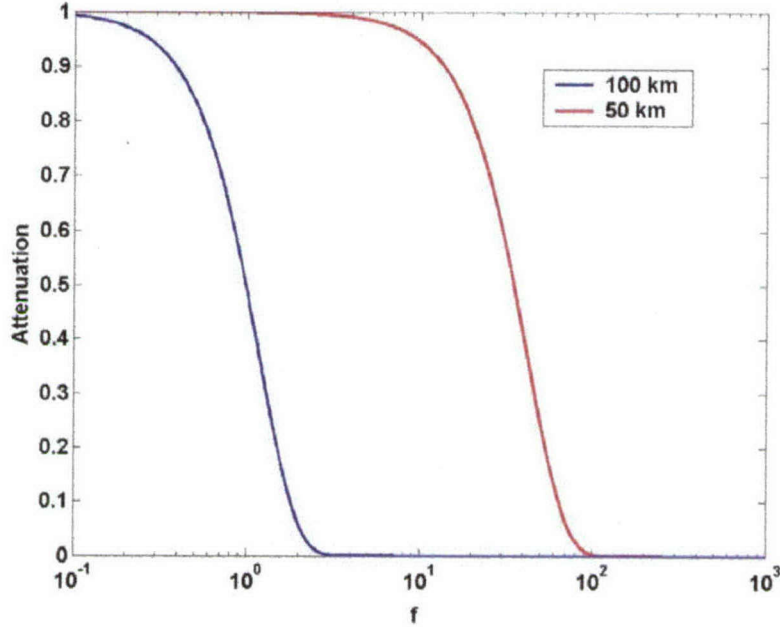
Figure 11: Attenuation as a function of frequency (in Hz) for scattering into the 50- and 100-km ducts.
