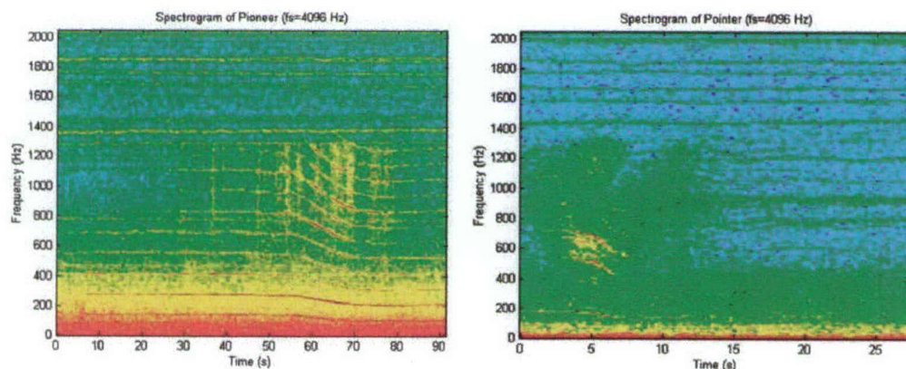
Figure 5: Left panel: acoustic power spectrum as function of time, for gasoline-powered UAV. Right panel: same, for electric-powered UAV. Source: Dr. S. Tenney, ARL.
