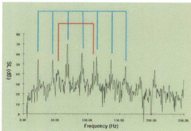
Figure 2: Acoustic power spectrum of a truck, from S. Tenney, ARL. The red lines represent narrowband signals from tire noise. The turquoise lines represent harmonics generated by the firing of the engine’s cylinders.
