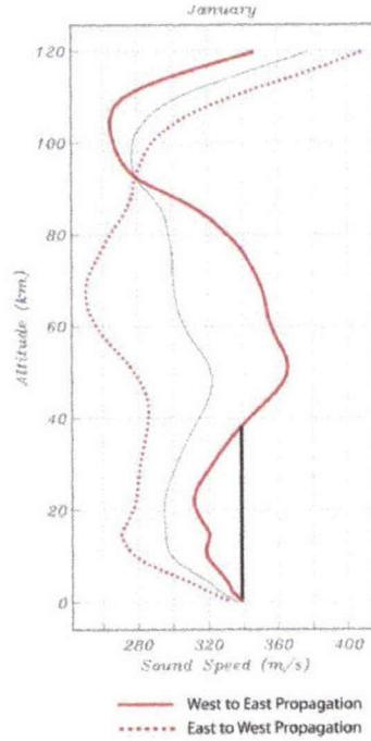
Figure 9: Sound speed vs. elevation in windy conditions. From ([34]
