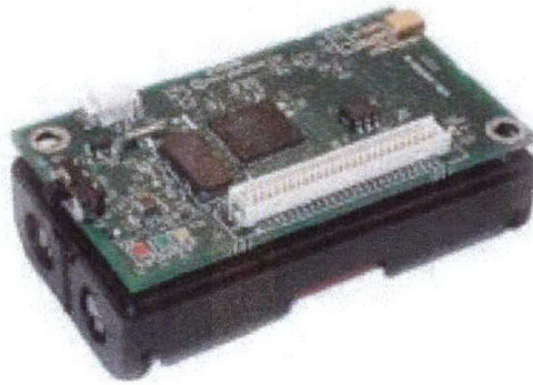
Figure 20: The Crossbow MICA2 wireless node
