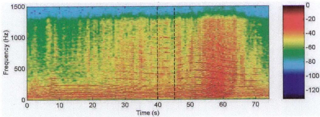
Figure 4: Sound intensity as a function of frequency and time, for a UH-1 helicopter flying past the acoustic detector. From S. Tenney, ARL.
