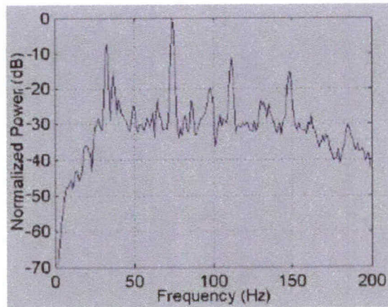
Figure 3: Acoustic power spectrum of an M60 tank, normalized to its maximum signal. From S. Tenney, ARL.
