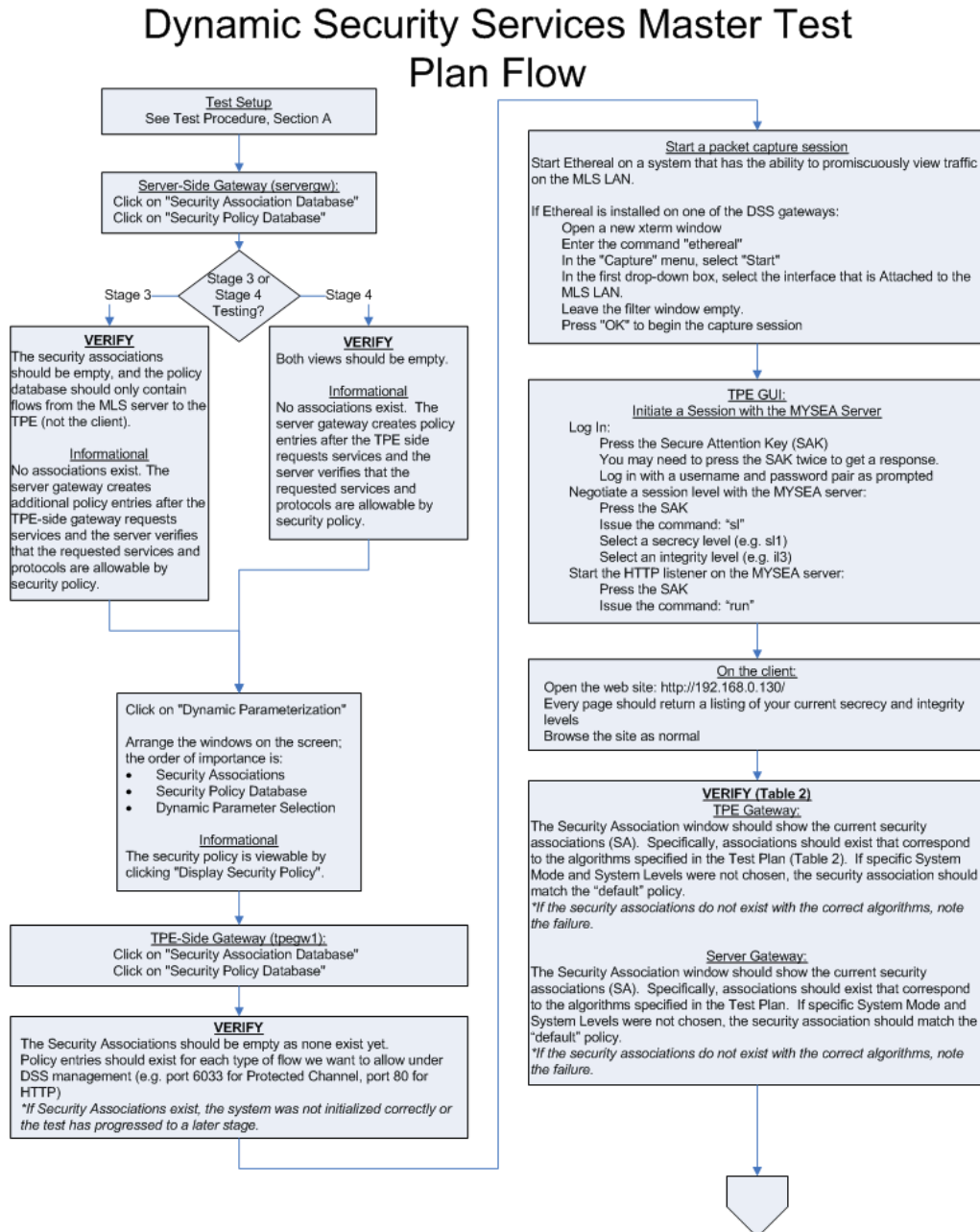
Figure 11. Test Procedure Flowchart, Part 1
