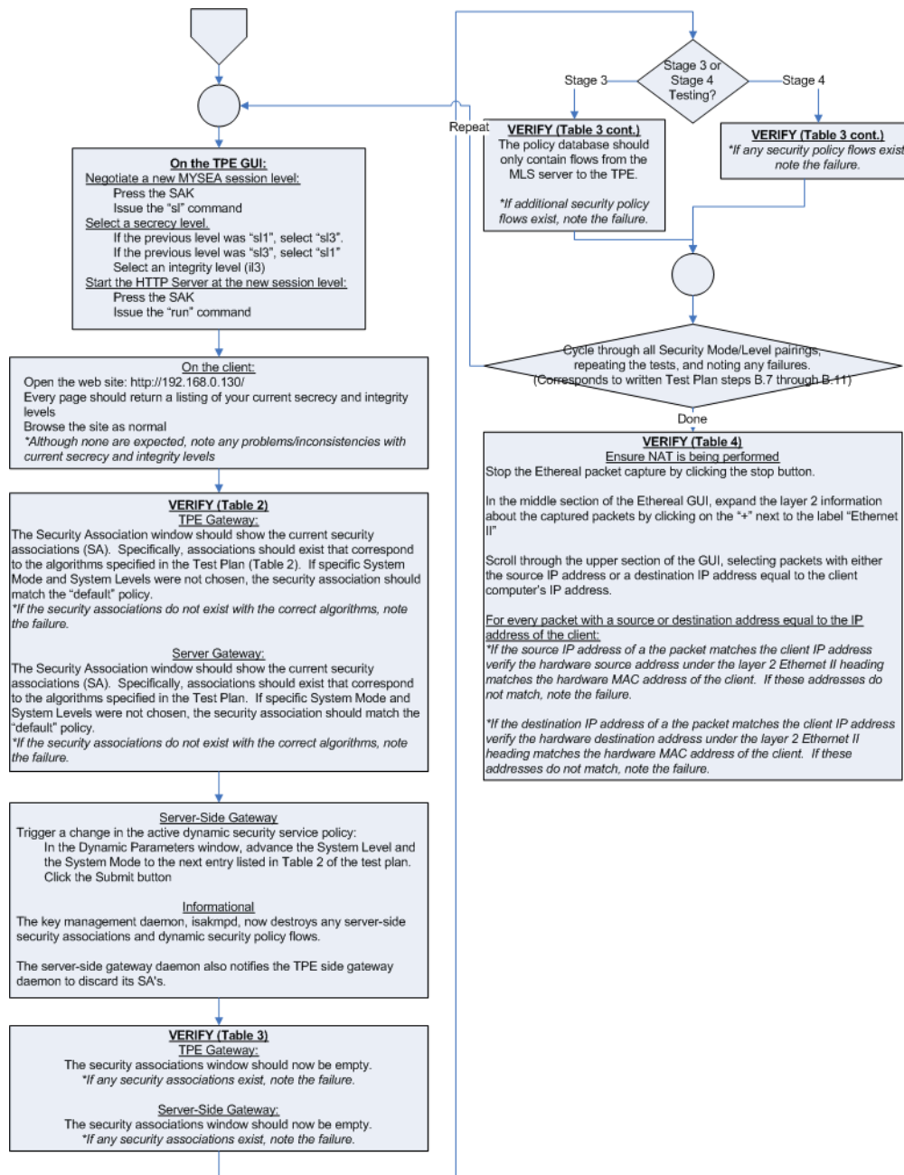
Figure 12. Test Procedure Flowchart, Part 2
