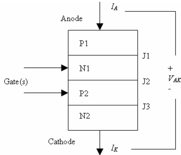
Figure 3. Thyristor Structure.
