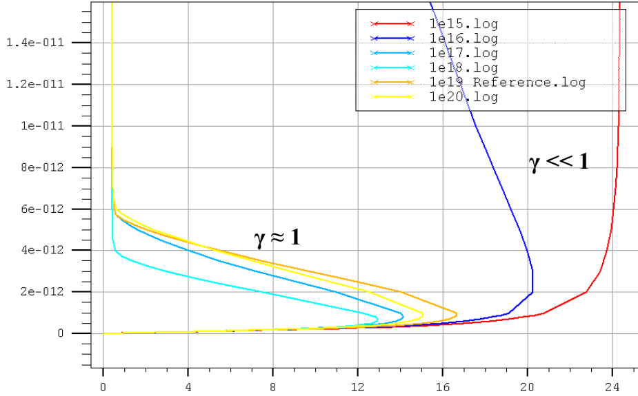
Figure 32. Anode Current vs. Bias as the N2 Doping Parameter is Varied.
