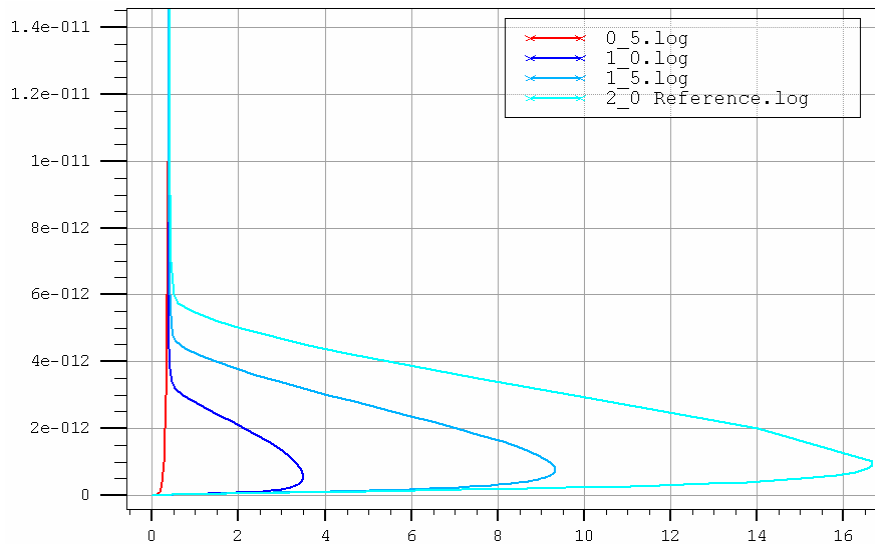
Figure 36. Anode Current vs. Bias as the N1 Thickness Parameter is Varied.
