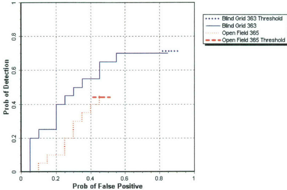
Figure 9. MAG TM-4/sling P_d^{disc} versus the respective P_{fp} for ordnance larger than 20 mm.
