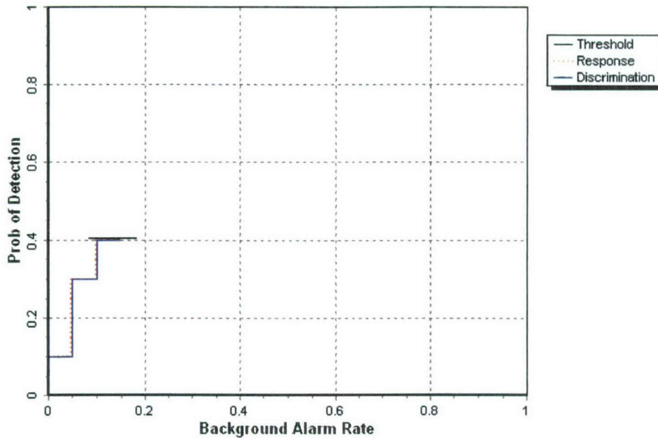
Figure 3. MAG (TM-4)/sling open field probability of detection for response and discrimination stages versus their respective background alarm rate over all ordnance categories combined.
