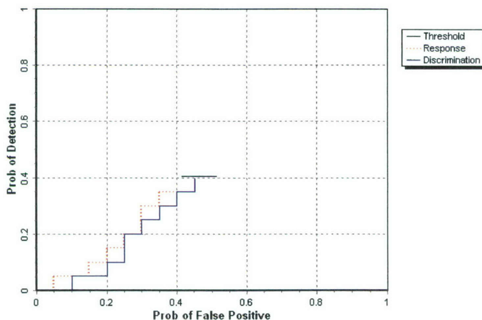
Figure 2. MAG (TM-4)/sling open field probability of detection for response and discrimination stages versus their respective probability of false positive over all ordnance categories combined.
