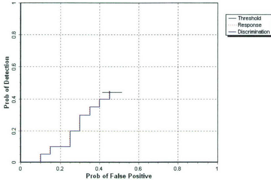
Figure 4. MAG (TM-4)/sling open field probability of detection for response and discrimination stages versus their respective probability of false positive for all ordnance larger than 20 mm.
