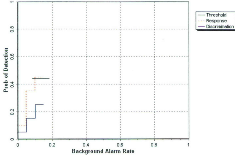
Figure 5. MAG (TM-4)/sling blind grid probability of detection for response and discrimination stages versus their respective background alarm rate for all ordnance larger than 20 mm.
