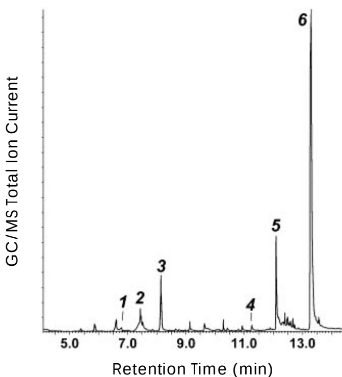
Figure 4-3. Ammonia GC/MS-Cl chromatogram of VX subjected to alkaline hydrolysis; Compound key for Figures 3, 4a, 4b, and 6: 1 O, S,-diethylmethylphosphonothiolate a , 2 2-(diisopropylamino)ethanethiol b , 3 2-(diisopropylamino) ethylmethyl sulfide a , 4 VX b , 5 bis(diisopropylaminoethyl)sulfide b , 6 bis(diisopropylaminoethyl)disulfide b . a Identification based upon apparent Cl pseudo-molecular ion only.
