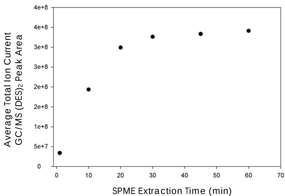
Figure 4-2. GC/MS-EI total ion current peak area for (DES) 2 plotted against SPME sampling time (PDMS fiber, 100 °C)
