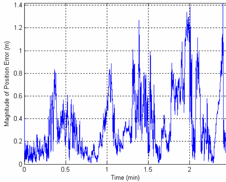
Figure III-9 Position error with decoy release.
