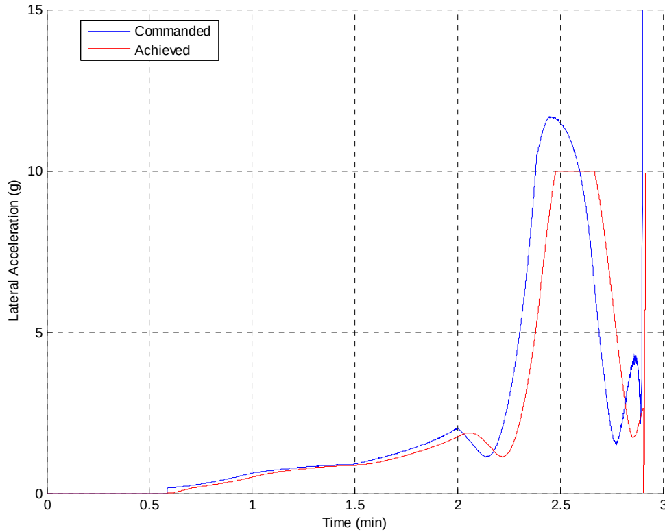
Figure IV-19 The no-EA case lateral acceleration for the MTT algorithm with a 35-second-delay launch.
