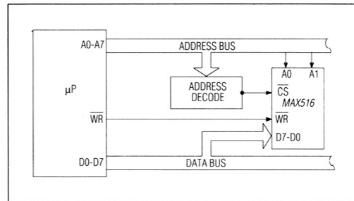
Figure 5. Microprocessor Interface
