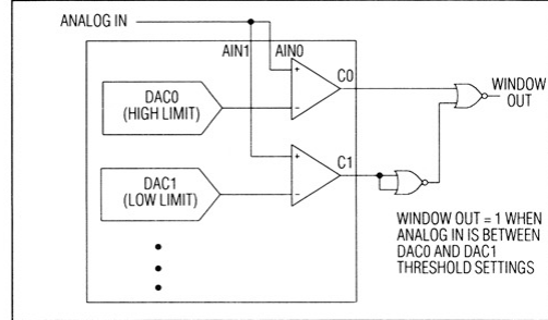
Figure 4. Window Comparison
