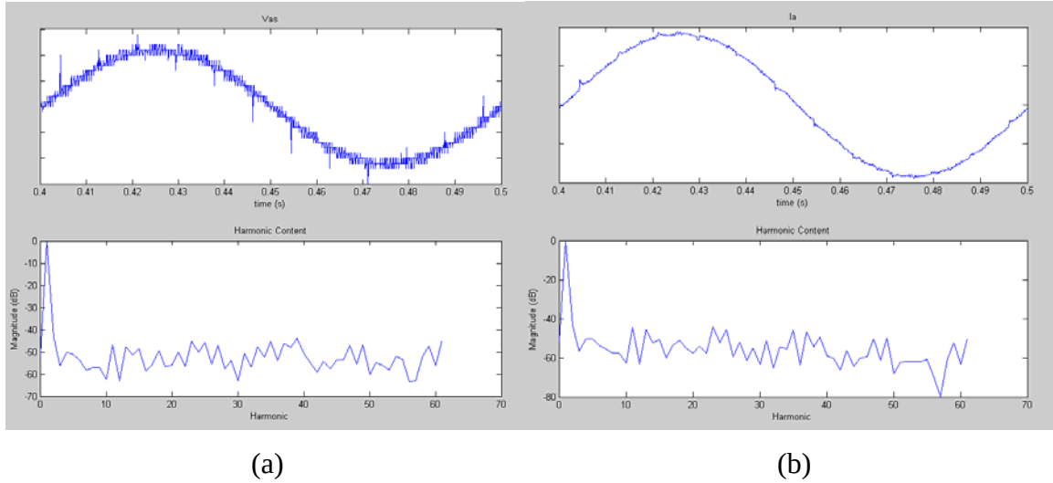
Figure E-3. (a) Output Voltage and (b) Output Current for 3x3 CMLC Simulations
