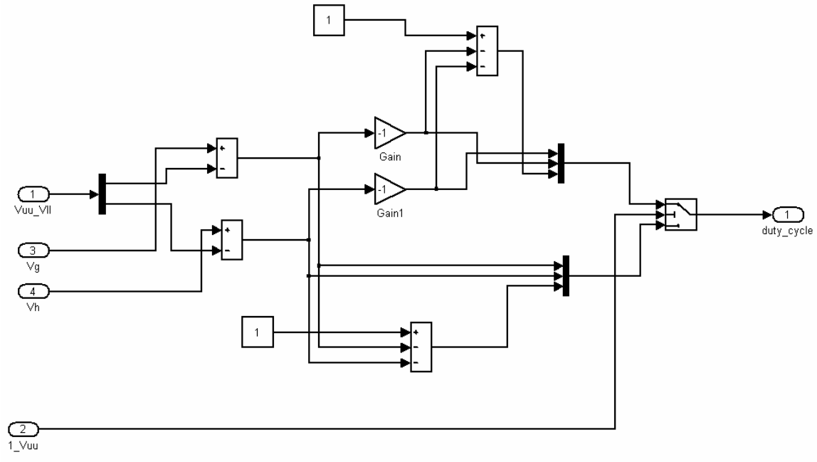
Figure 39. Calculation of Duty Cycles
