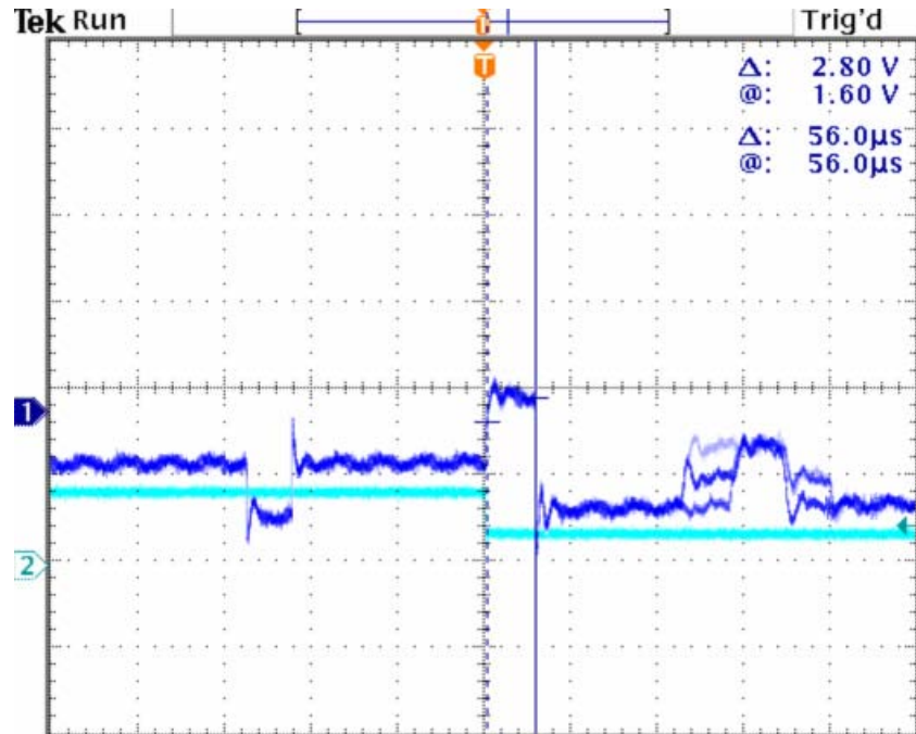
Figure 65. Voltage Spike for Hybrid Algorithm
