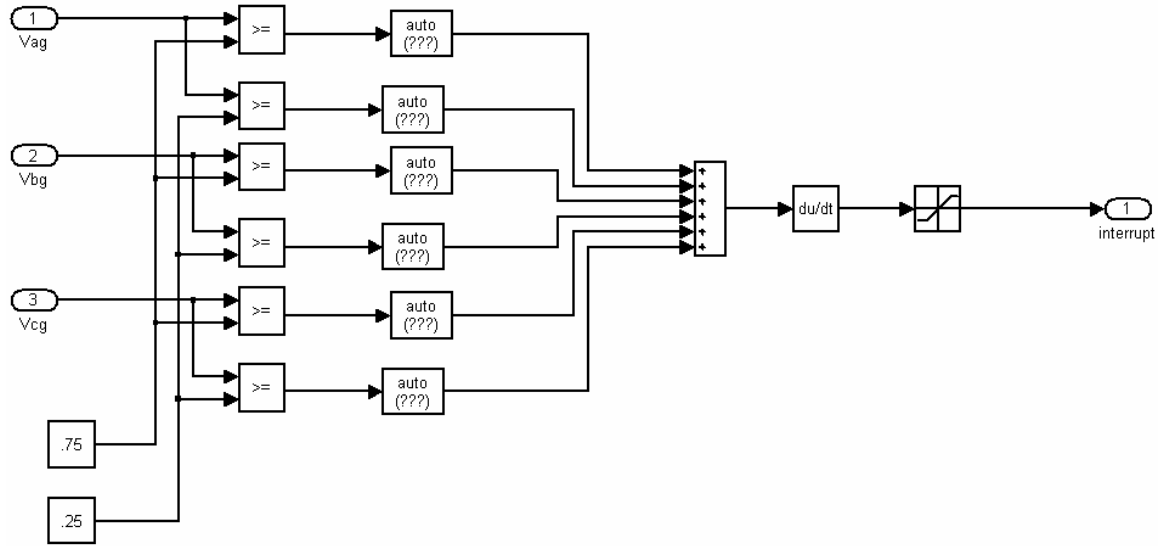
Figure 37. Software-Reset Block
