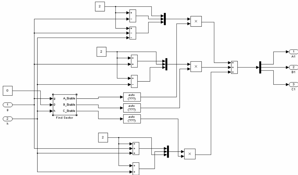
Figure 45. Hybrid Algorithm
