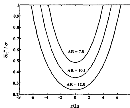
Fig. 12. Average axial normal stress in the matrix.
