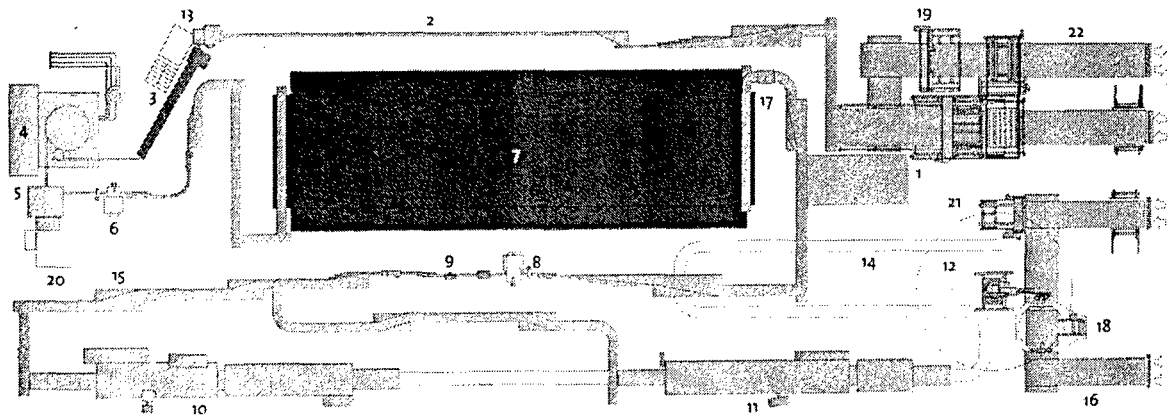
1 pushing device, 2 cable transport, 3 rinsing machine, 4 can filler, 5 can closure, 6 filling level control, 7 pasteurizer, 8 filling level control, 9 Inkjet dating, 10 six packer, 11 tray packer, 12 palletizer, 13 tin separator, 14 trade unit transport, 15 box transport, 16 palette transport, 17 pressure-relief station, 18 palette stretcher, 19 empty palette magazine, 20 shears stroke table, 21 palette magazine, 22 palette transport
