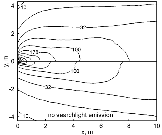
Figure 6. Comparison of the net radiative energy flux with and without searchlight emission. Values are in \text{W/m}^2 .
