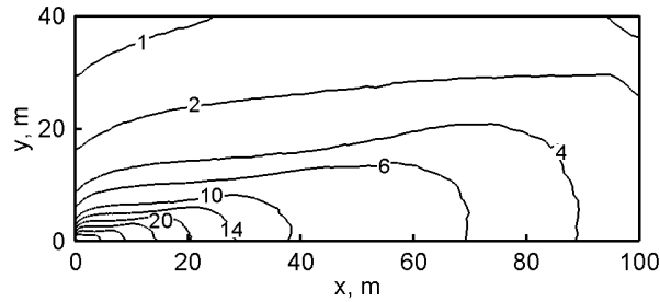
Figure 5. Contours of the net direction-averaged radiative energy flux. Values are in \text{W/m}^2 .
