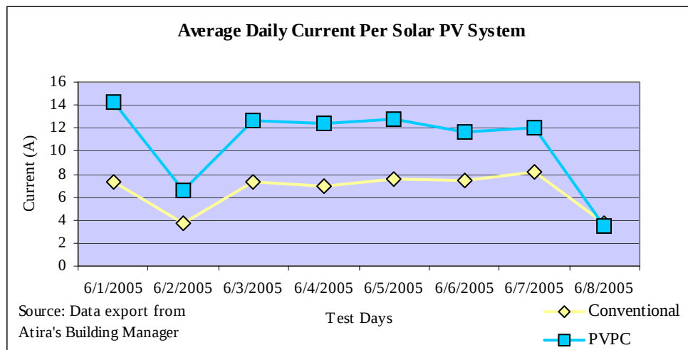
Figure 21 Total Average Daily Current for each Solar PV System.
