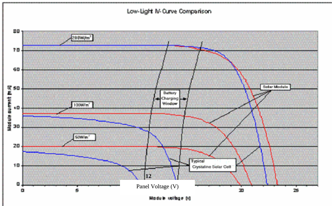
Figure 15 Low Light Effect on Battery Charging. (From www.solengy.com/pages/whitepapers.html , April 2005)
