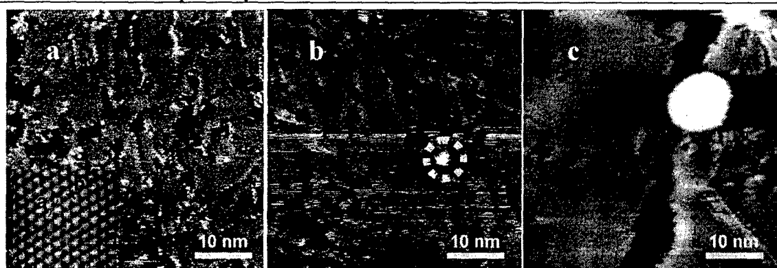
Figure 26: Constant current STM topography of a dodecanethiolate SAM on Au (111)/mica, before (a) and after (b) the insertion of 6 ; the molecule is shown as bright spot and indicated by a circle. c. The image of the surface after attachment of Au nanoparticle to the top termini of 6 . The area showed is 50 \times 50 \text{ nm}^2 , STM imaging conditions: V_{\text{bias}} = +1.0 \text{ V} , I_t = 1 \text{ pA} ).
