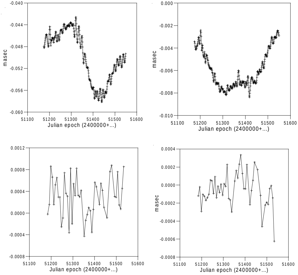
Figure 1. Corrections to IAU 1980 nutation model in \Delta\psi (top, left) and \Delta\epsilon (top, right) and to Herring's nutation model (bottom, left) and \Delta\epsilon (bottom, right).
