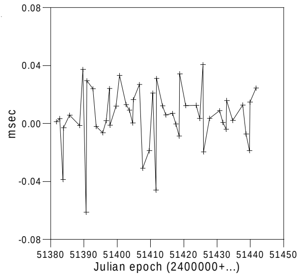
Figure 3. Variations of UT1–UTC from NEOS-Intensives using Herring's nutation model.
