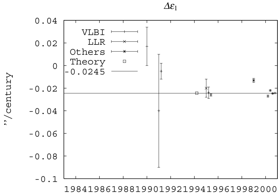
Figure 3. Corrections to Precession in Obliquity.
