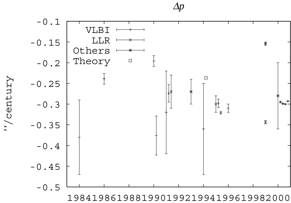
Figure 1. Corrections to Precession in Longitude
