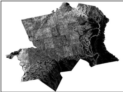
Figure 24. Physical slope, Fort Bragg region.
