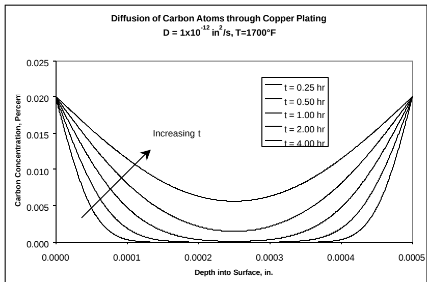
Figure 17 – Model of carbon diffusion through copper plating (0.0005 inch). Similar curves could be generated using different values of D (estimated) and t . (a) Assuming infinite
