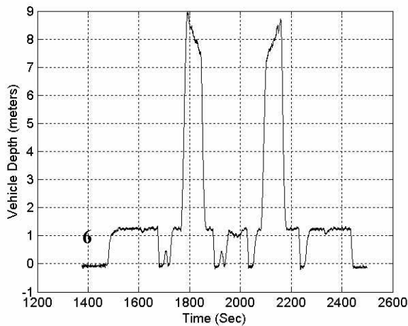
Figure 5a. Vehicle Path showing locations where the GPS position fixes were obtained by surfacing for 20 seconds (asterisks). 5b. Depth response during run that clearly shows the DGPS pop up maneuvers.
