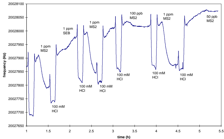
Figure 1. Sensor response of plasmopolymerised BAW crystals coated with anti-MS2 antibodies on injections of 1 \mu\text{g}/\text{ml} MS2 in HBS and 1 \mu\text{g}/\text{ml} SEB (control of specificity); 100 \mu\text{l} sample injection in carrier flow rate of 25 \mu\text{l}/\text{min} .
