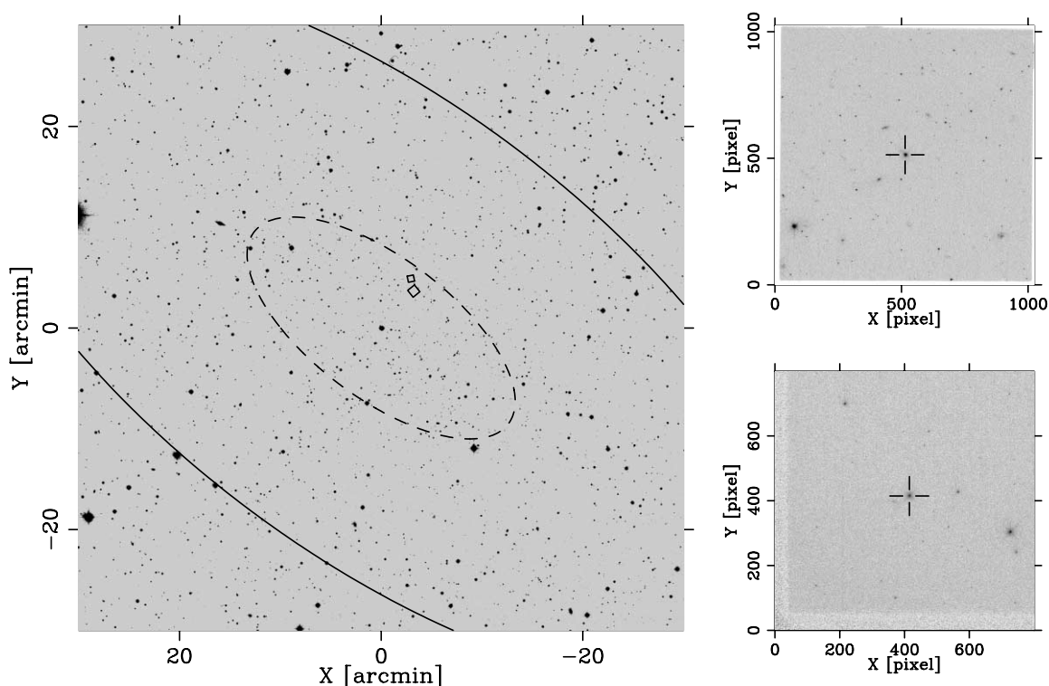
FIG. 1.— Left : Image of the sky in the direction of the Ursa Minor dSph. The dashed ellipse is the measured core radius, and the solid ellipse is the measured tidal boundary. The two squares represent the fields studied in this article. The larger of the two corresponds to the UMI J1508+6716 field, and the smaller to the UMI J1508+6717 field. Top right : Sample image from the epoch 2000 data for the UMI J1508+6716 field. The cross-hair indicates the location of the QSO. Bottom right : Sample image from the epoch 1999 data for the UMI J1508+6717 field. Again, the cross-hair indicates the location of the QSO.
