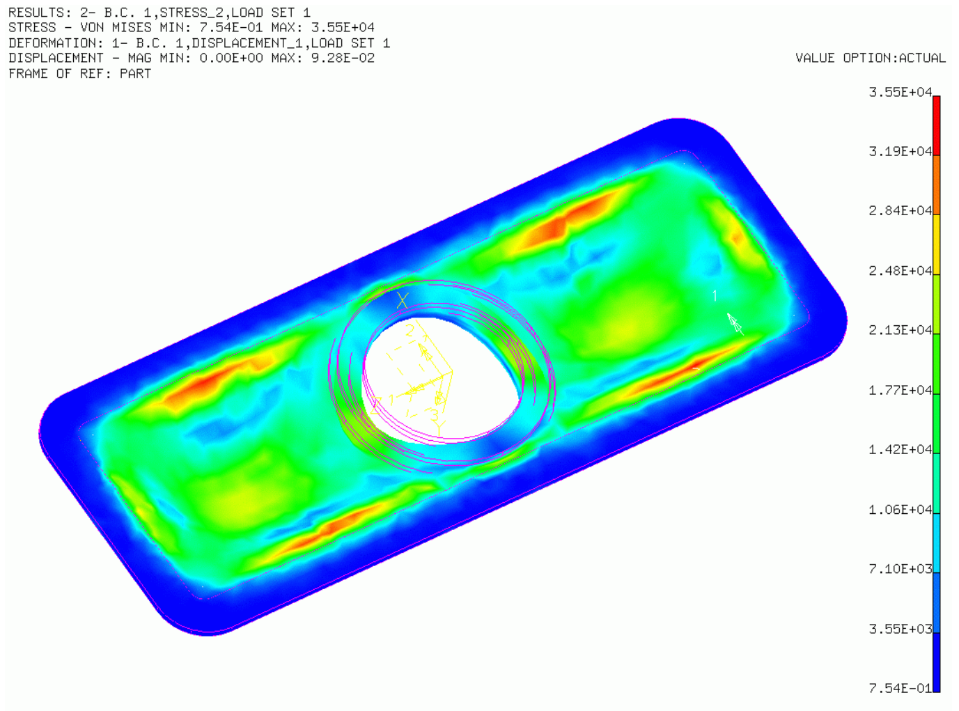
Figure VI -1 : Von Mises stress plot of the hatch plate at 300feet
