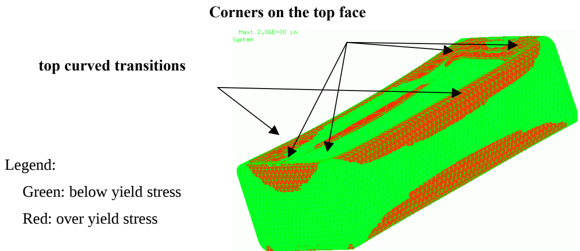
Figure VI -4 : Von Mises stress plot of the hull at 300feet Isometric view
