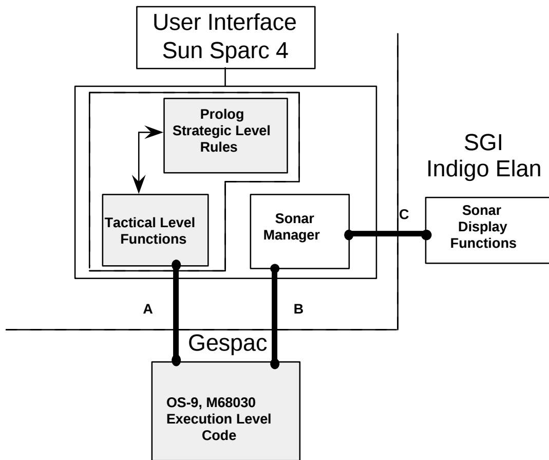
Figure 2 Outline Of The Phoenix Networked Controller
