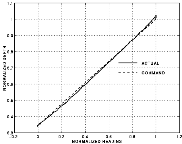
Figure 7. Normalized Depth vs. Heading Response
