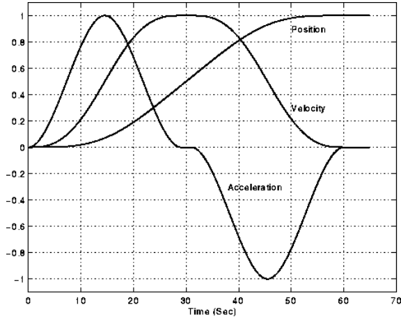
Figure 4. Normalized Command Generator Profiles
