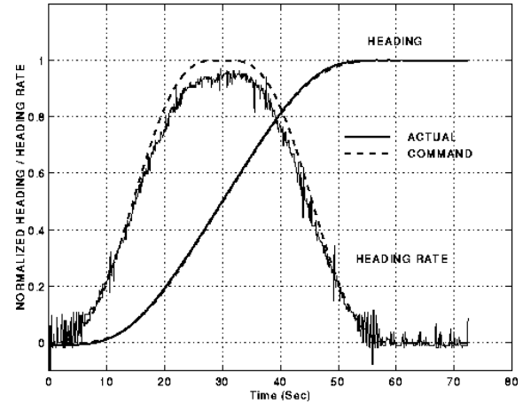
Figure 6. Normalized Heading and Heading Rate Response
