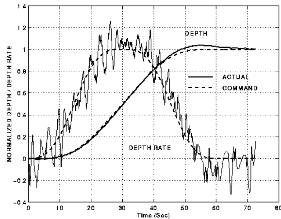
Figure 5. Normalized Depth and Depth Rate Response
