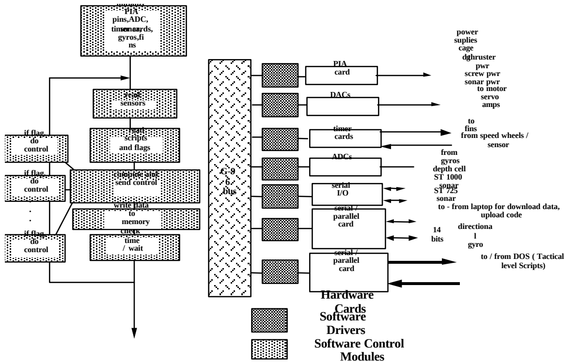
Diagram of the Software / Hardware Interface of the Execution Level of the NPS ATIV II
