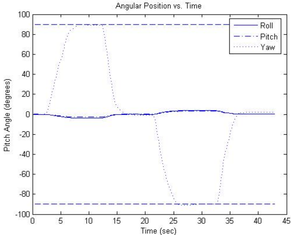
Figure 11. Rotation Test: Angular Position vs. Time
