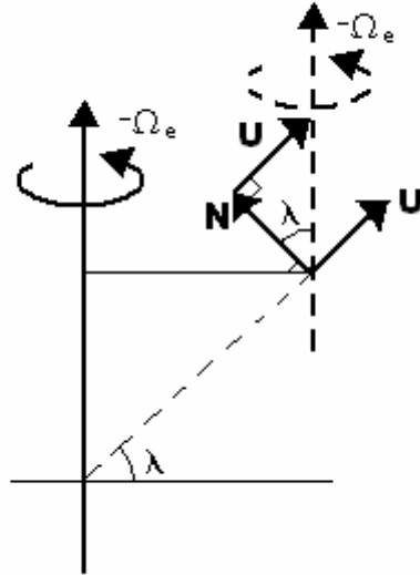
Figure 13. Shifted Earth Rotation Axis
