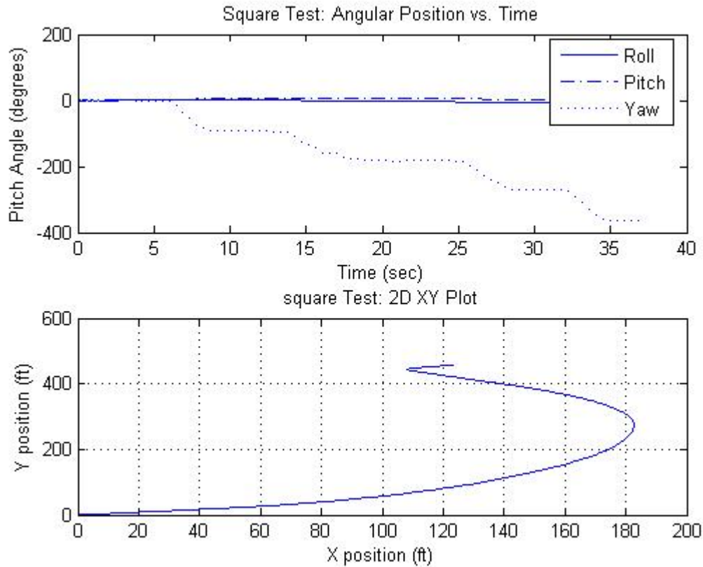
Figure 18. Positioning Test: Square Route
