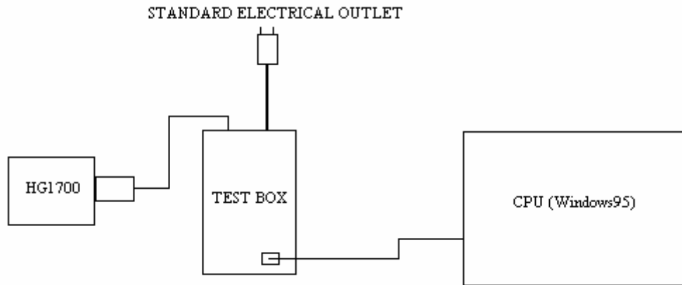
Figure 3. Test Box Block Diagram
