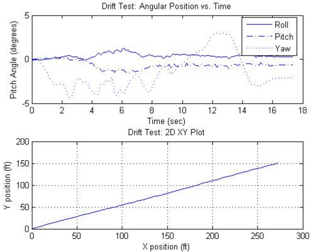
Figure 20. Positioning Tests: Drift Route
