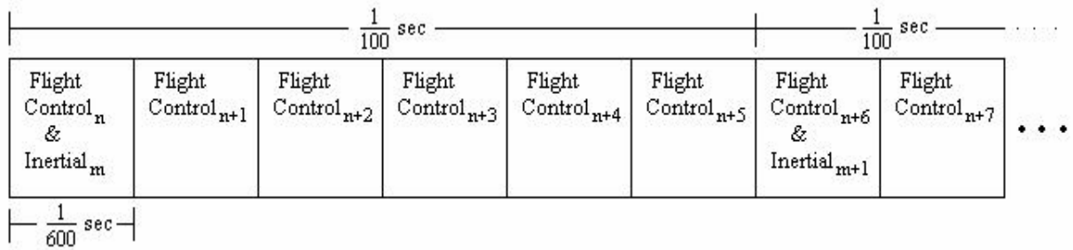
Figure 8. IMU Rate of Measurement and Transmission (After Ref. [5])
