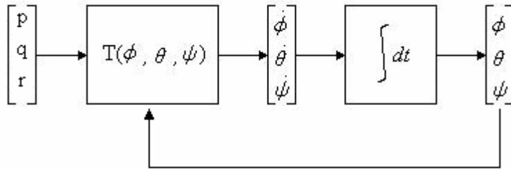
Figure 16. Euler Angle Loop
