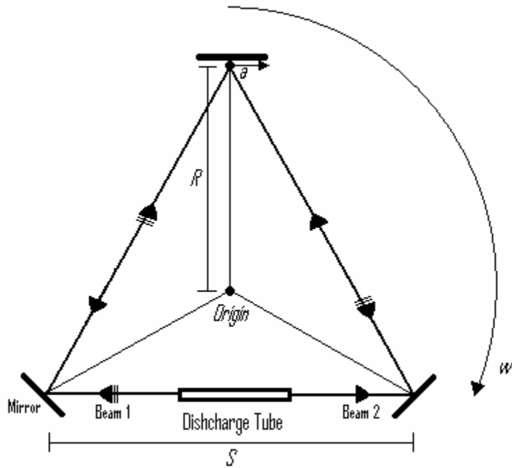
Figure 1. Equilateral Triangle (After Ref. [4])
