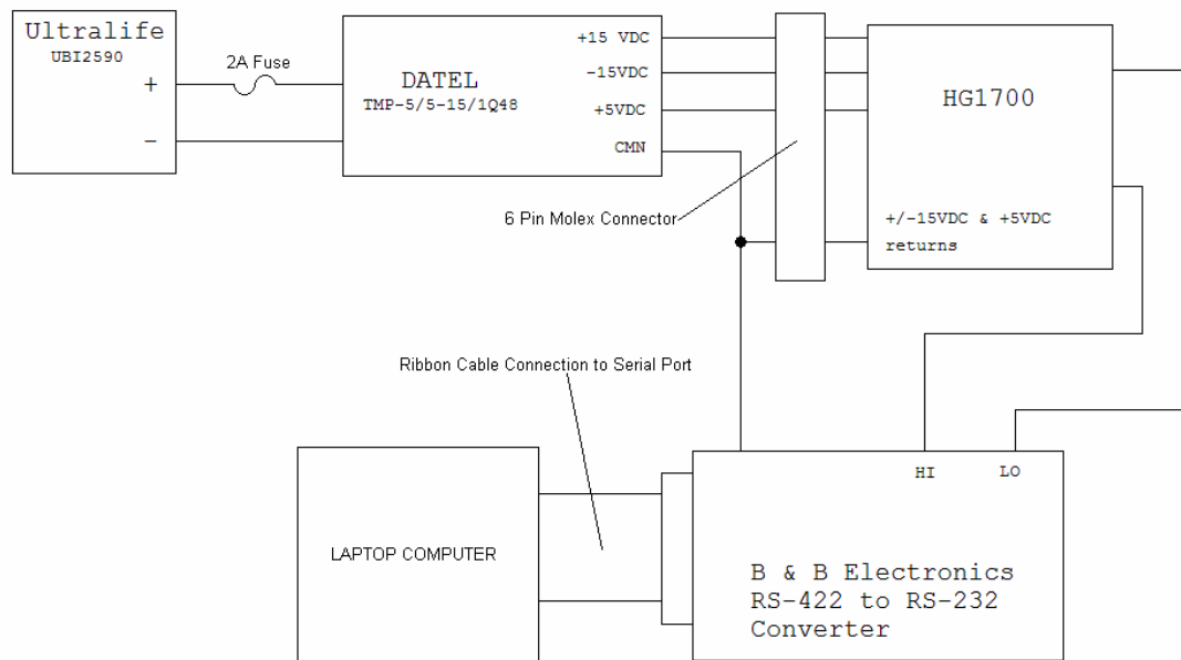
Figure 5. C++ Block Diagram
