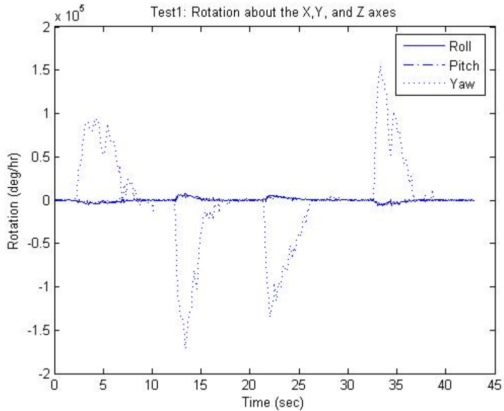
Figure 10. Rotation Test: Rotation Rates vs. Time
