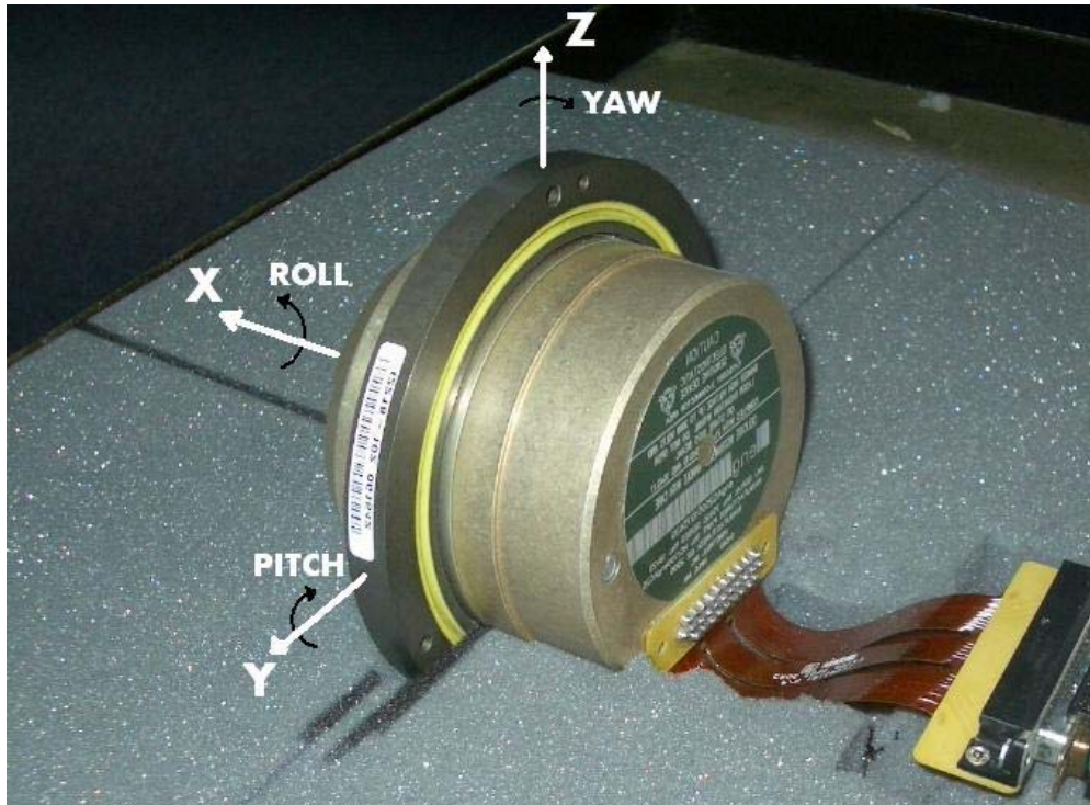
Figure 7. Photo Orientation of IMU
