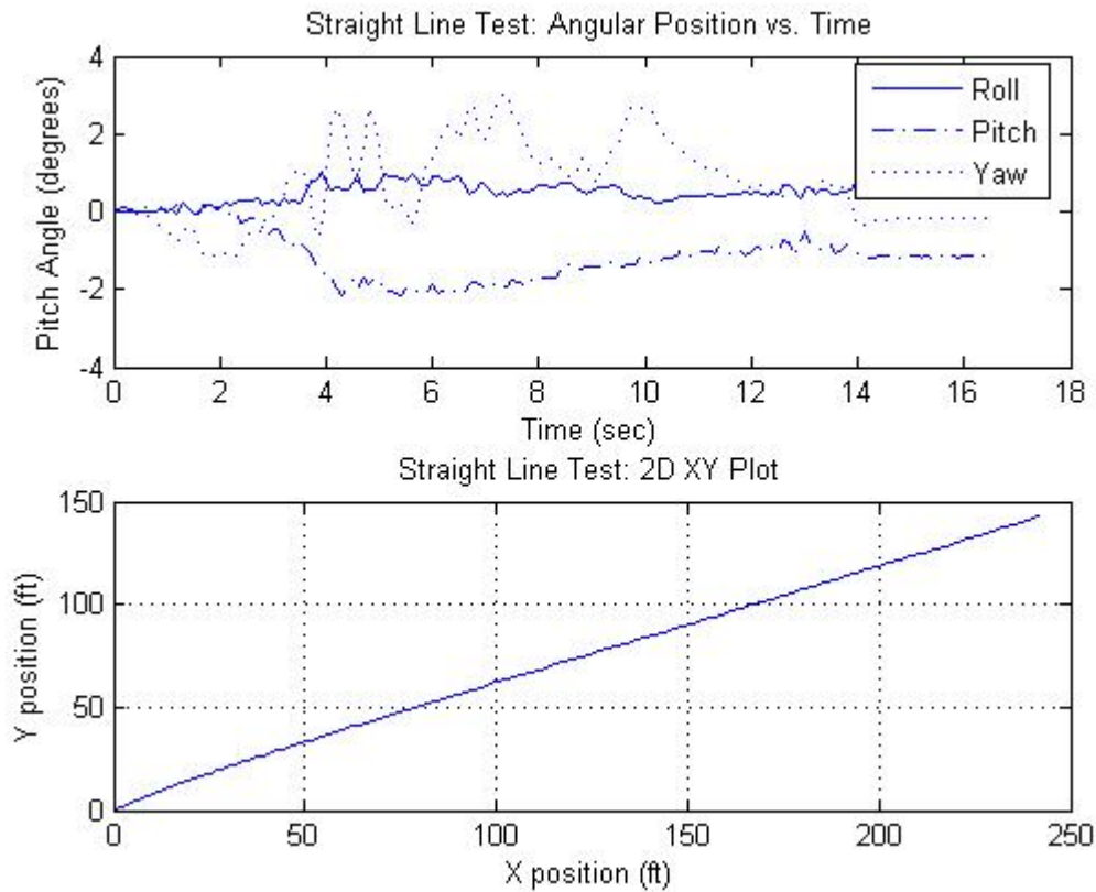
Figure 19. Positioning Tests: Straight Route
