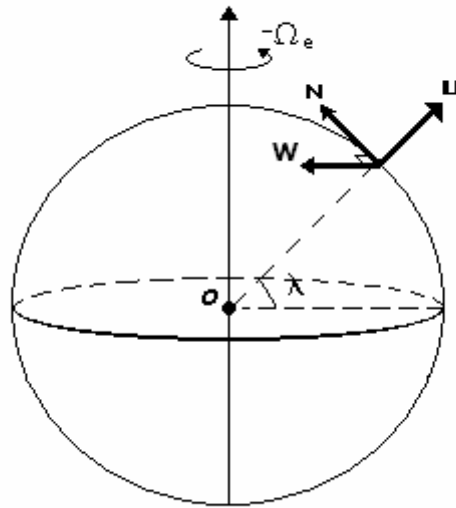
Figure 12. Earth Rotation
