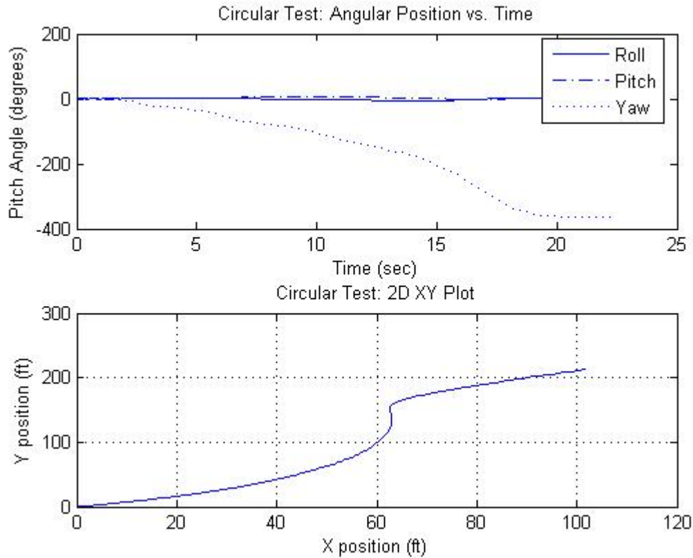
Figure 17. Positioning Tests: Circular Route
