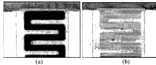
Fig. 3: Optical micrographs of MSM Photodetector devices (a) nanostructured and (b) planar.
