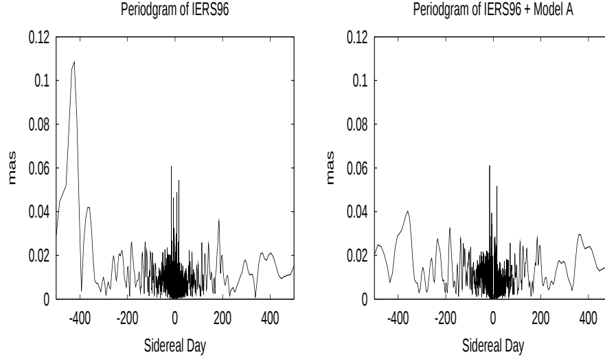
Figure 2. Spectra of Complex Residuals for IERS96 Nutation Theory with and without FCN. The strong peak in the spectrum of the IERS96 nutation theory around -400 sidereal days is clearly removed by adding a model FCN term.
