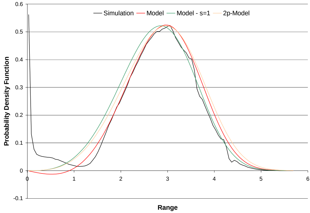
Figure 15. Probability density function of the stress ranges and its approximations by Eq. (B.25) (“Model”), Eq. (B.26) (“Model - s = 1 ”), and Eq. (B.28) (“2p- Model”), SPL = 144 dB.
