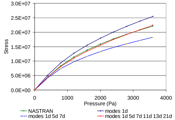
Figure 3. Static response of an unbuckled panel to a uniform pressure. Stress \sigma_{xx} as a function of pressure.
