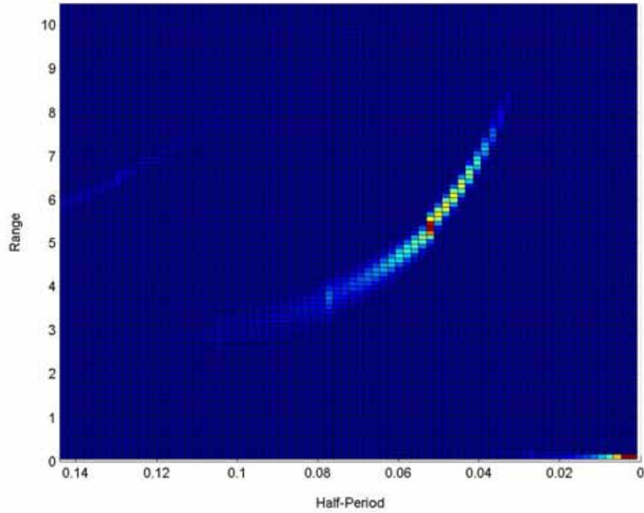
Figure 10. Two-dimensional histogram of ranges and half-periods, SPL = 154 dB
