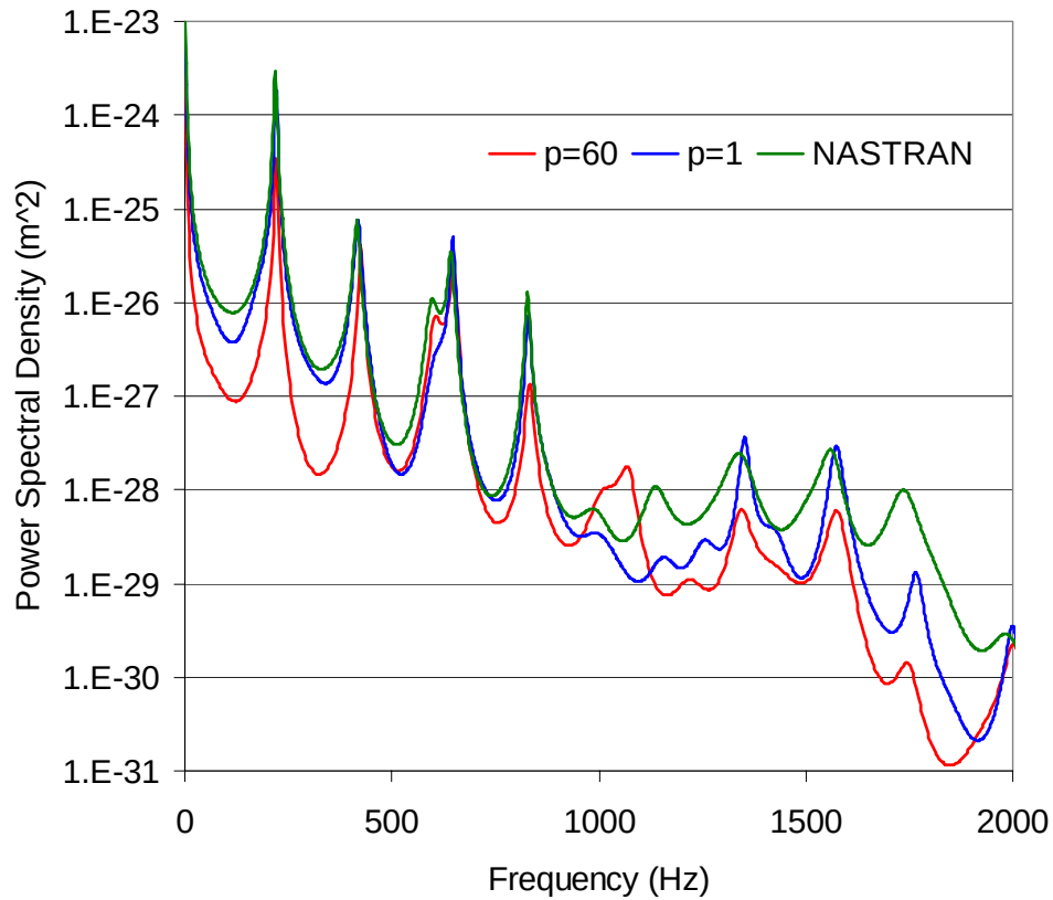
Figure 15. In-plane x-displacement spectrum for aluminum panel, SPL = 97dB , computed from MSC.NASTRAN and ELSTEP/FAT with 8 modes and duals, p = 60Pa and p = 1Pa .
