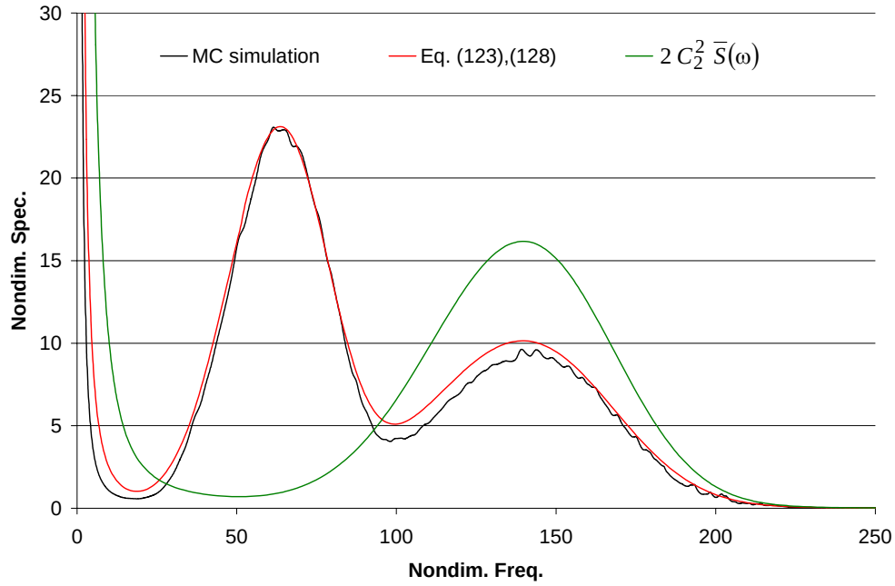
Figure 5. Comparison of stress spectra computed by Monte Carlo simulations of Eq. (1), (2), and (116) (“MC simulation”), and by using the method of Appendix A with either Eq. (121) or Eq. (123) and (128).
