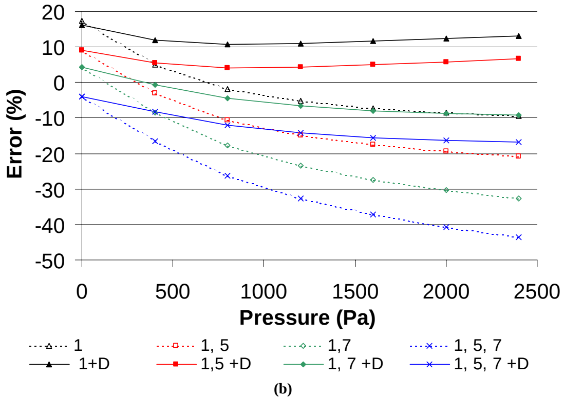
Figure 6. Reduced order modeling errors in the static response of panel 2 to a uniform pressure for different number of modes with (“+D”) and without duals. (a) Center displacement and (b) stress \sigma_{xx} at center as functions of pressure.
