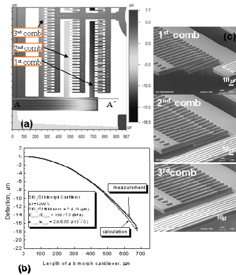
Figure 96. Biomorph cantilever.
