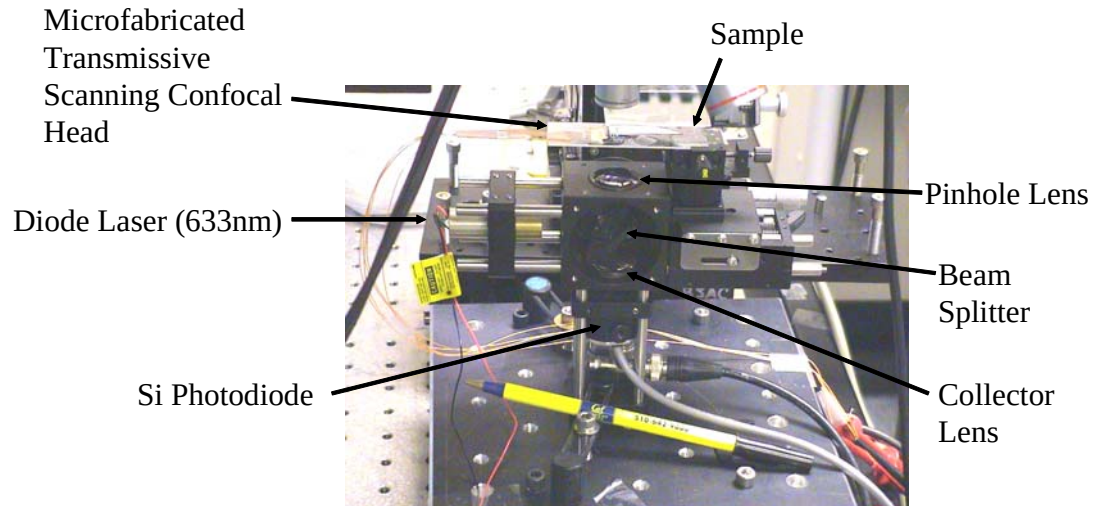
Figure 109. Photograph of the miniaturized laser scanning confocal microscope.
