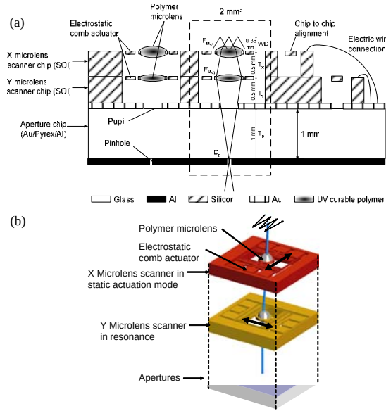
Figure 20. (a) Device architecture of the micromachined transmissive scanning microscope, and (b) Schematic diagram of the transmissive raster scanning.
