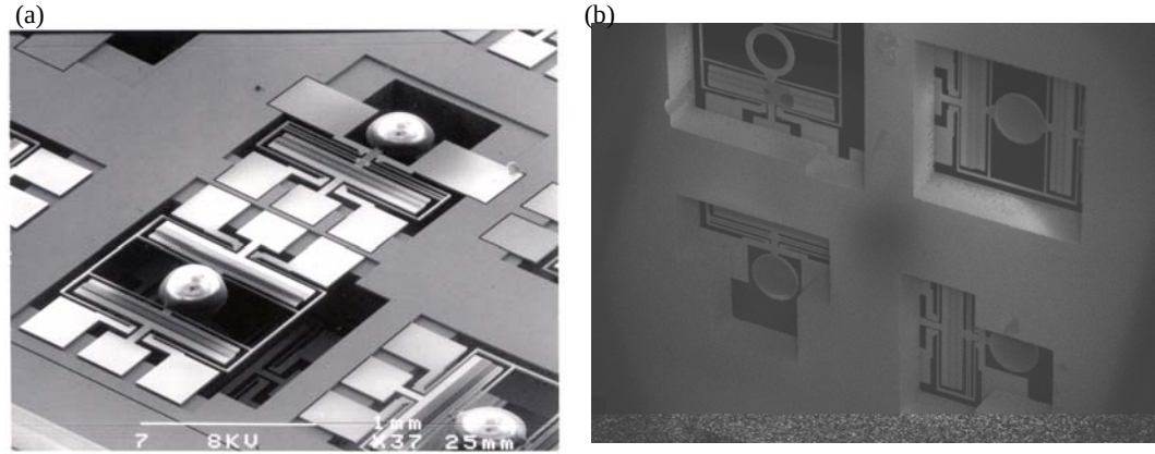
Figure 32. SEM micrographs of microlens scanners taken (a) from the top, and (b) from the bottom.
