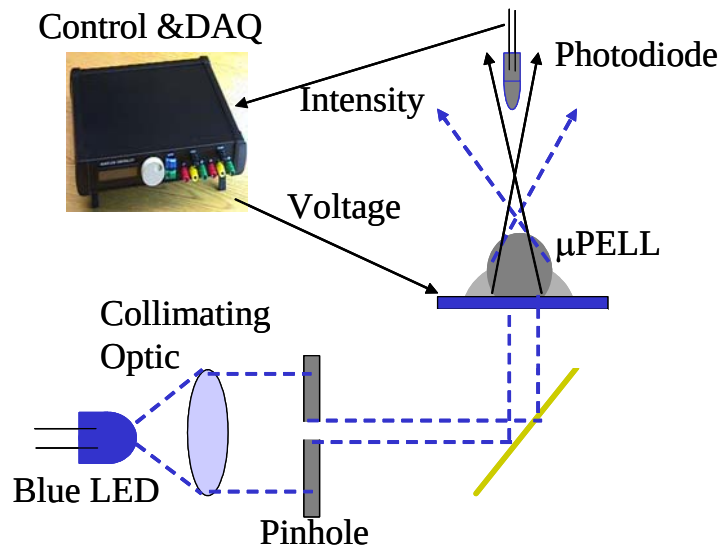
Figure 85. Experimental setup for dynamic measurements of the focal length change.
