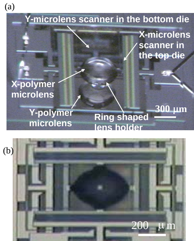
Figure 33. SEM micrographs (a) of a stacked 2-D microlens scanner, and (b) of a top view.
