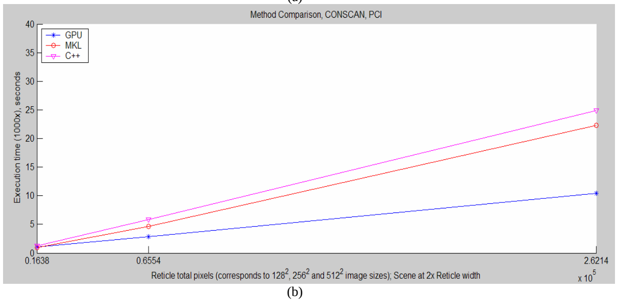
Figure 5-3. Conical scan execution times compared for the GPU and CPU-based Processing Methods, at the three image sizes, and on both (a) AGP, and (b) PCI-express platforms. Plots show same information contained in Table 5-7 above.
