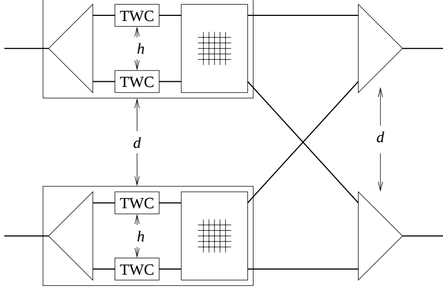
Figure 3: Wavelength converting switch using Tunable Wavelength Converters (TWC), Optical Crossbars and Passive Multiplexors and Demultiplexors
