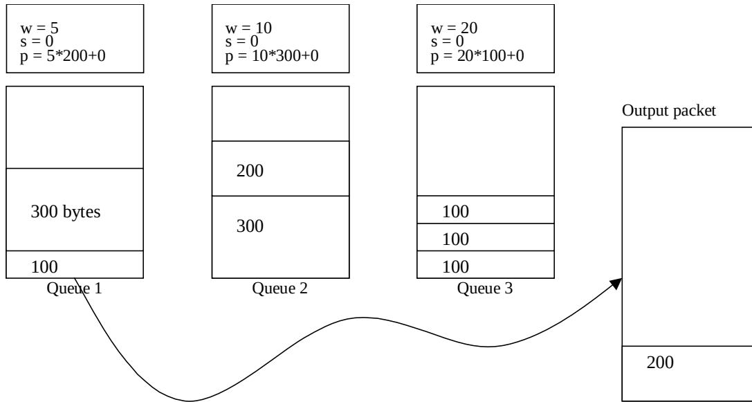
Figure 18: Queue 1 has the minimum provisional score; therefore, its first packet gets stuffed into the output buffer.
