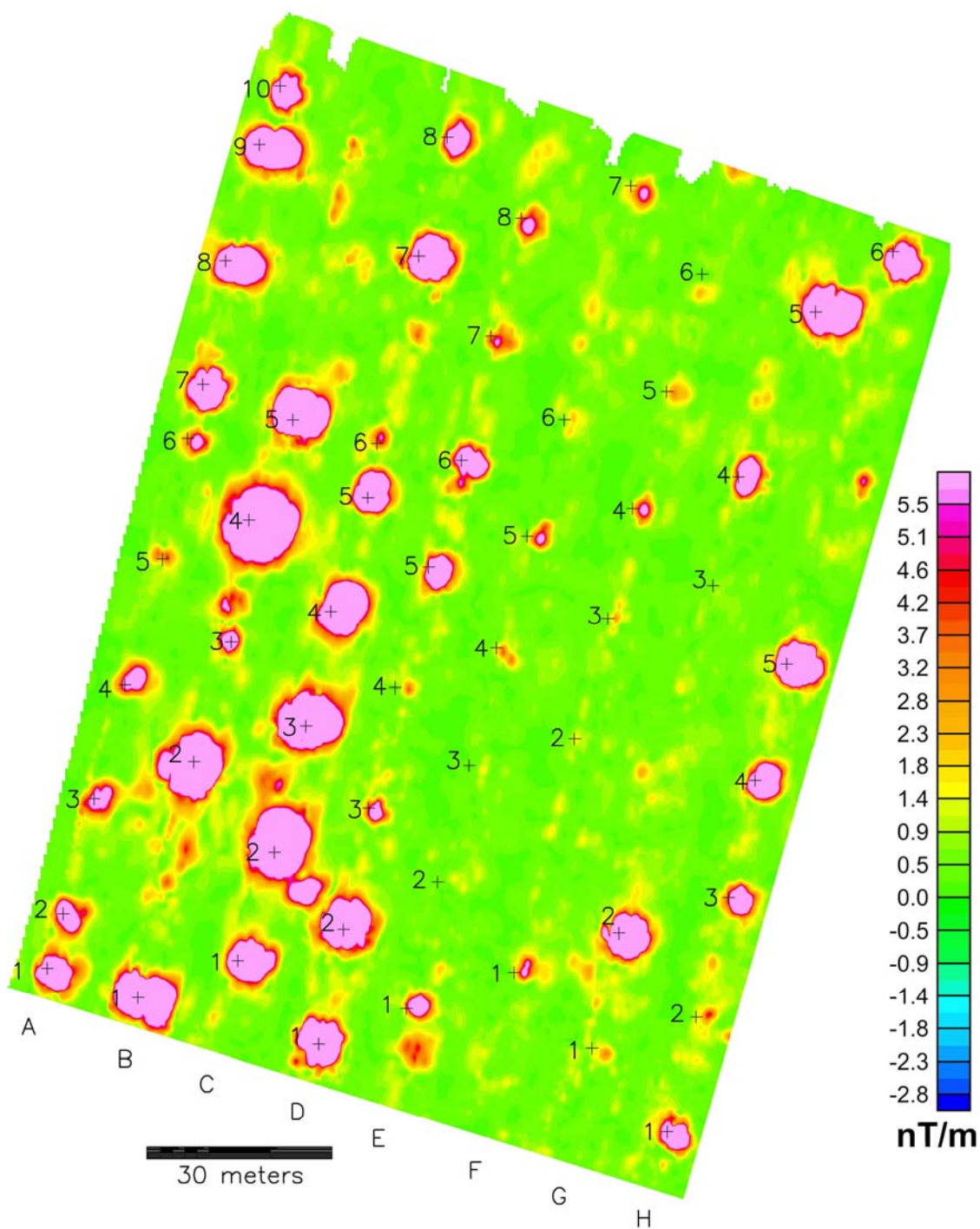
Figure 23. Analytic signal map derived from airborne (ORAGS-Arrowhead) magnetic data, BBR Test Site, September 2002, for comparison with EM results.
