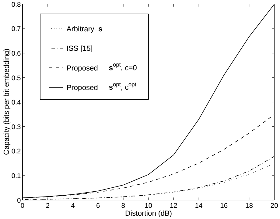
Fig. 5. Capacity versus distortion (Baboon image, \sigma_n^2 = 3\text{dB} ).
