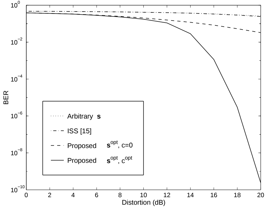
Fig. 4. Bit-error-rate versus host distortion (Baboon image, \sigma_n^2 = 3\text{dB} ).
