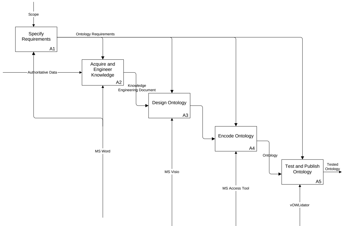
Figure 3. Ontology Development Process
