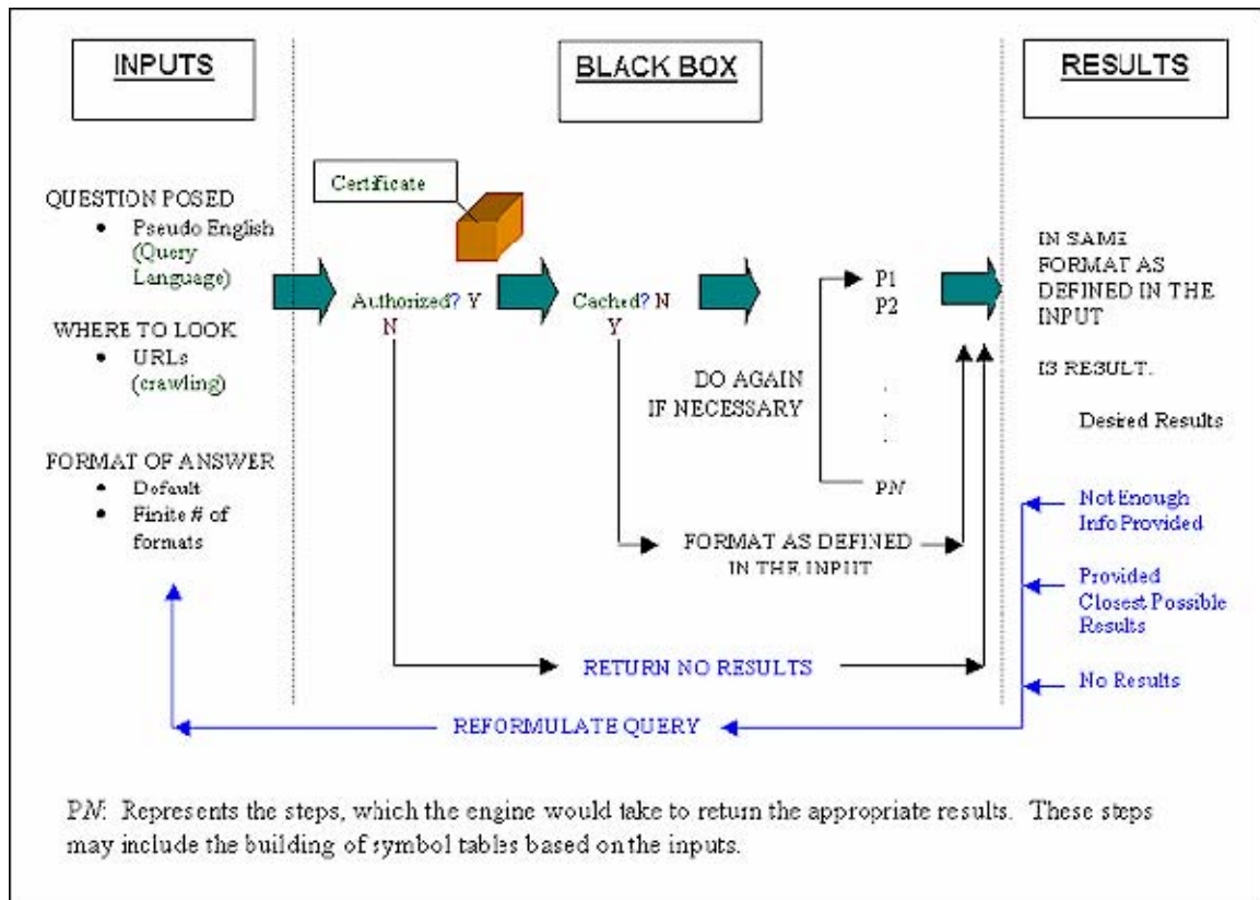
Figure 2. Query Lifecycle
