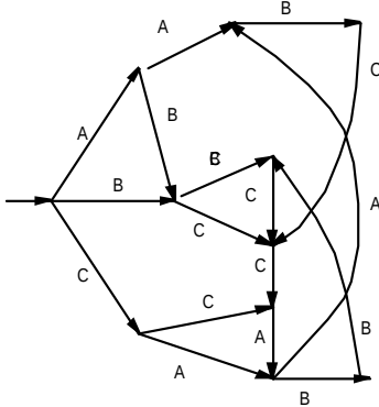
Figure 5. Automaton resulting from compression of Figure 2
