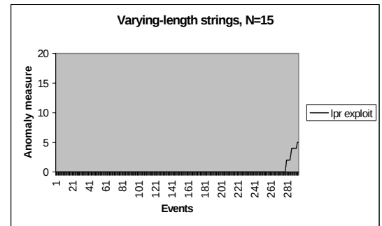
Figure 8. Multiple-length strings (max length = 15) for lpr exploit
