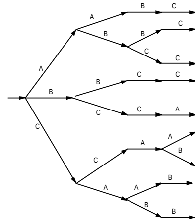
Each node at depth k ( k \leq N ) in the tree is labeled with a k -gram of the training strings. The leaf nodes at depth N are labeled with N -grams (ABCC, ABBC, etc.). The root node is labeled with the empty string.
