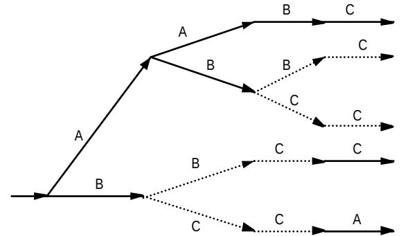
Figure 4. Redundant portions of (part of) the suffix tree
