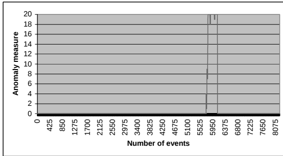
Figure 9. N-gram anomaly measure for inetd exploit ( N = 6 )
