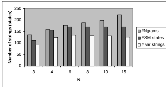
Figure 14. Growth of synthetic lpr database as function of N
