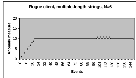
Figure 12. Rogue client, measured using multiple-length strings ( N = 6 )
