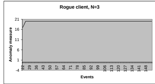
Figure 11. Rogue client, measured using N-gram method ( N = 3 )
