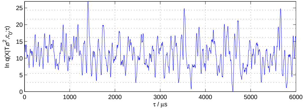
(a) q_{\mathcal{N}} -score with \sigma = 12\mu\text{s} , c_0 = -2.705 .
