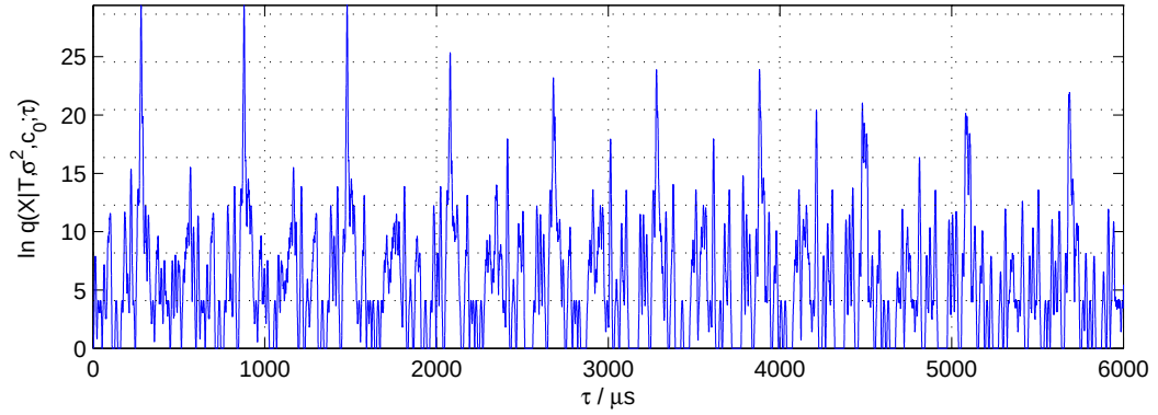
(a) q_{\mathcal{H}} -score with \sigma = 3\mu s , c_0 = -4.092 .
