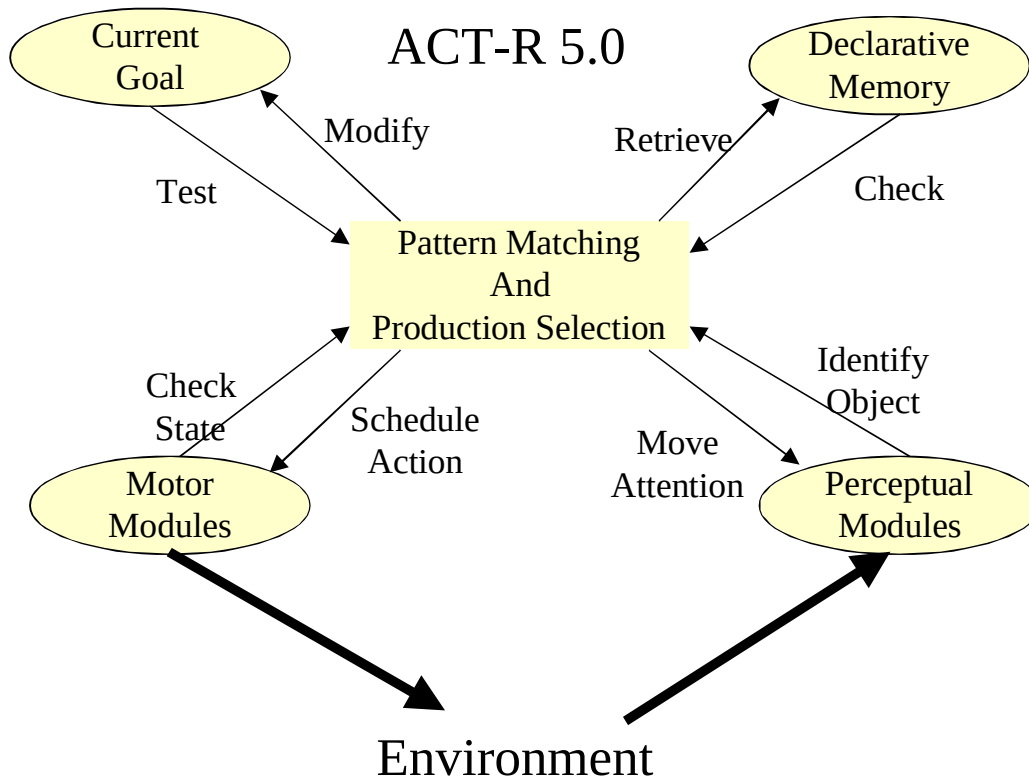
Figure 1. A schematic of the major components of ACT-R. Reprinted with permission of Lebiere.
