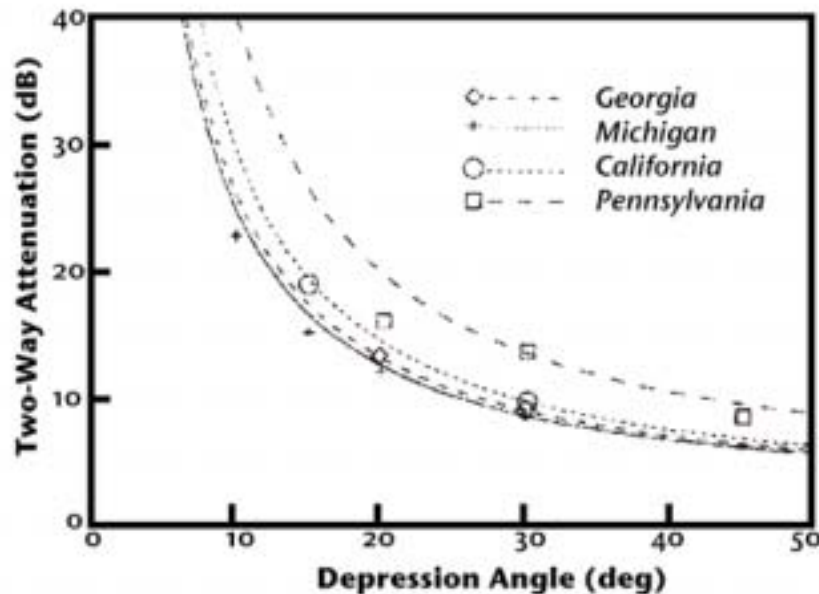
Figure 3. Variation of Two-Way Attenuation (UHF) with Depression Angle (Bessette and Ayasli)
