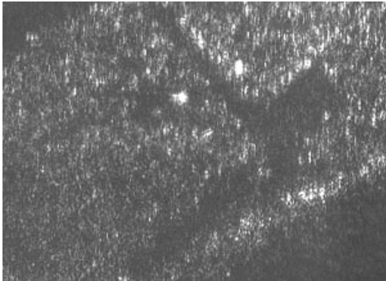
Figure 8. Examples of two 2x4m Flat Metal Panels under California Forest (one end-on, one broadside, SCR is +17 and +20dB)
