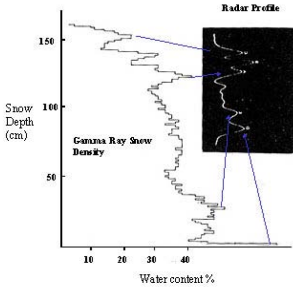
Figure 9. A Radar Profile through Alpine Snowpack (1972) at 2200 MHz. (Vickers 1973)
