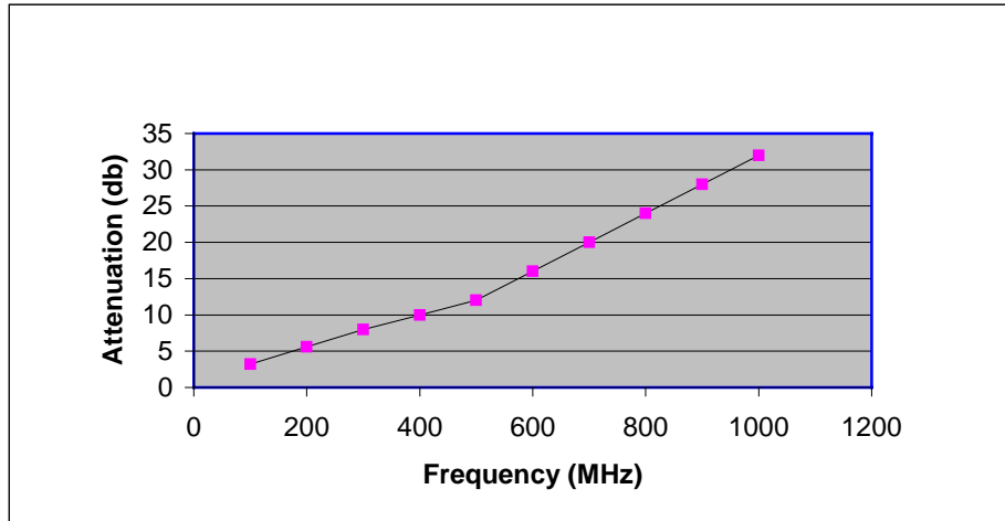
Figure 1. Two-Way Attenuation through Forest Canopy as a Function of Frequency
