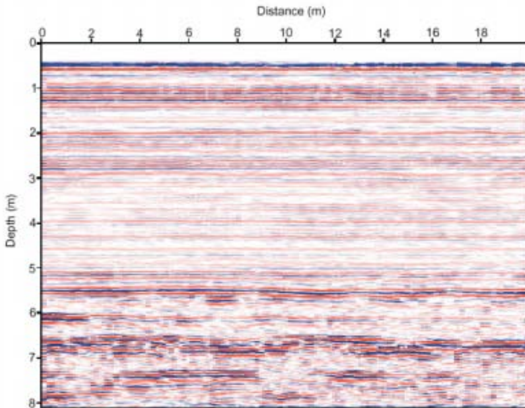
Figure 10. Vertical Profile through Dry Snowpack at 900 MHz showing Internal Layering despite Low Reflection Coefficients. (De Brabander 2003)
