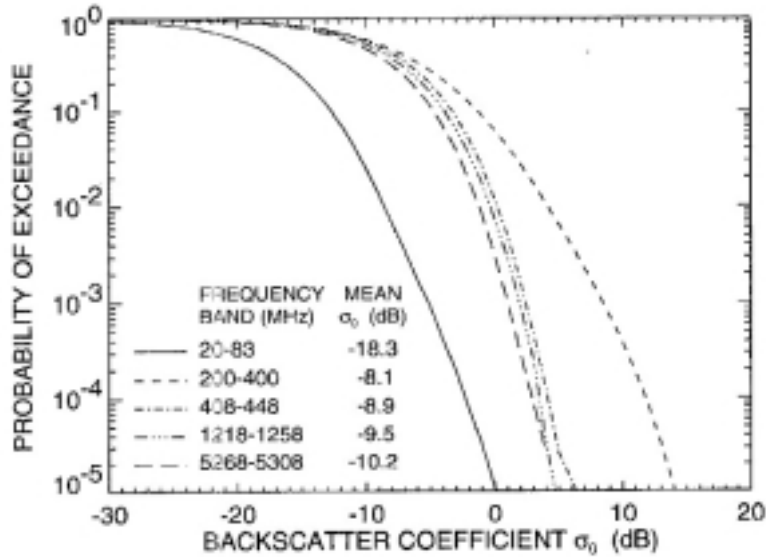
Figure 5. Exceedance Diagram for Backscatter from 20 – 5300 MHz
