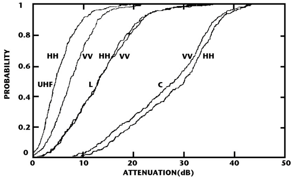
Figure 2. Cumulative Probability Distribution curves for Two-Way Attenuation at Three Radar Frequencies.
