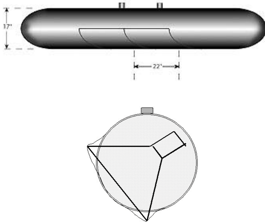
Figure 13. Possible Antenna Mounting in CC-130 Pod
