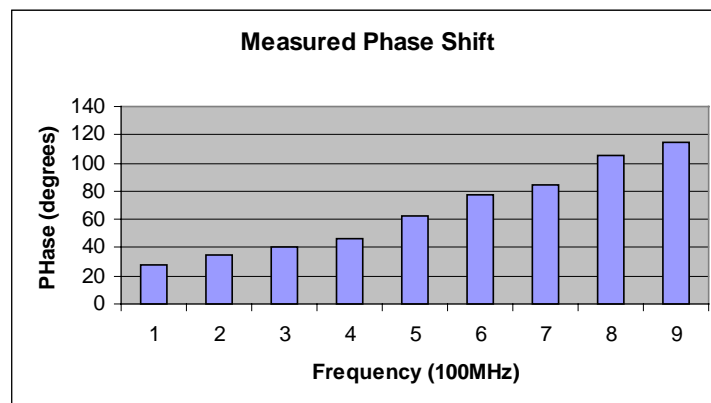
Figure 4. Phase Shift through Forest Canopy Vs Frequency
