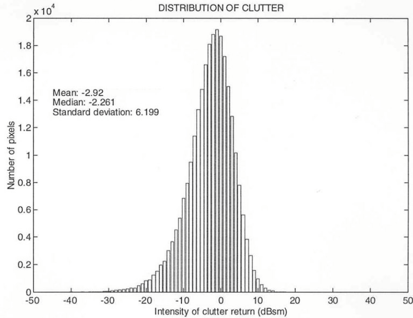
Figure 6. Clutter Distribution for Californian Forest, 200 – 400 MHz (Dreyer 1995)
