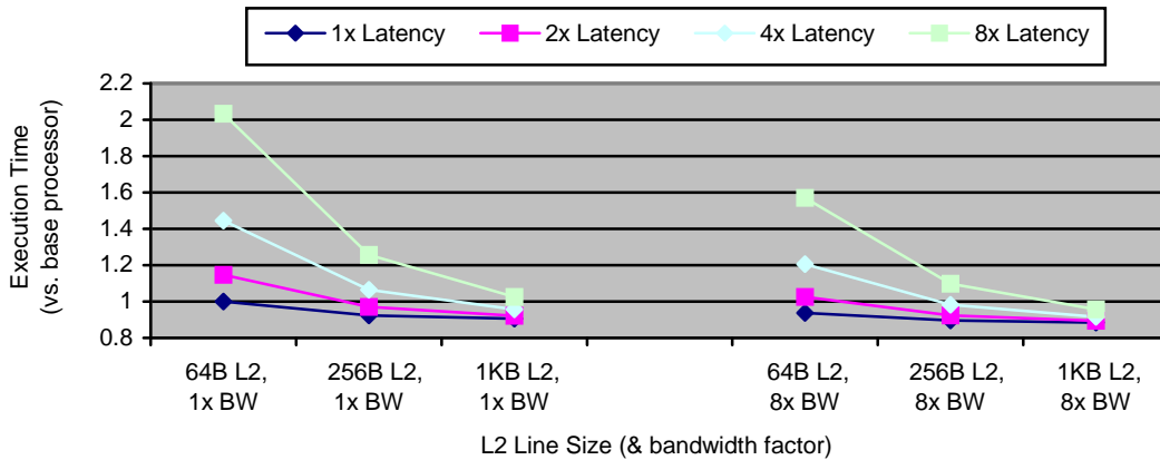
Figure 10. Average of latency and bandwidth vs. L2 line size using input-1 .
