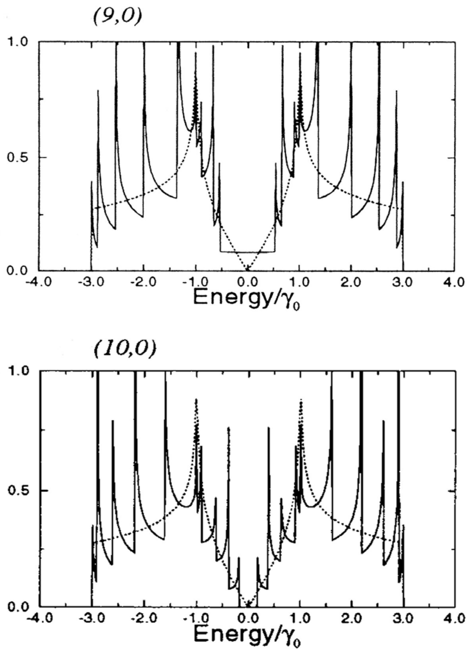
Figure 2. Calculated Electronic DOS for a (9, 0) and a (10, 0) Nanotube.
