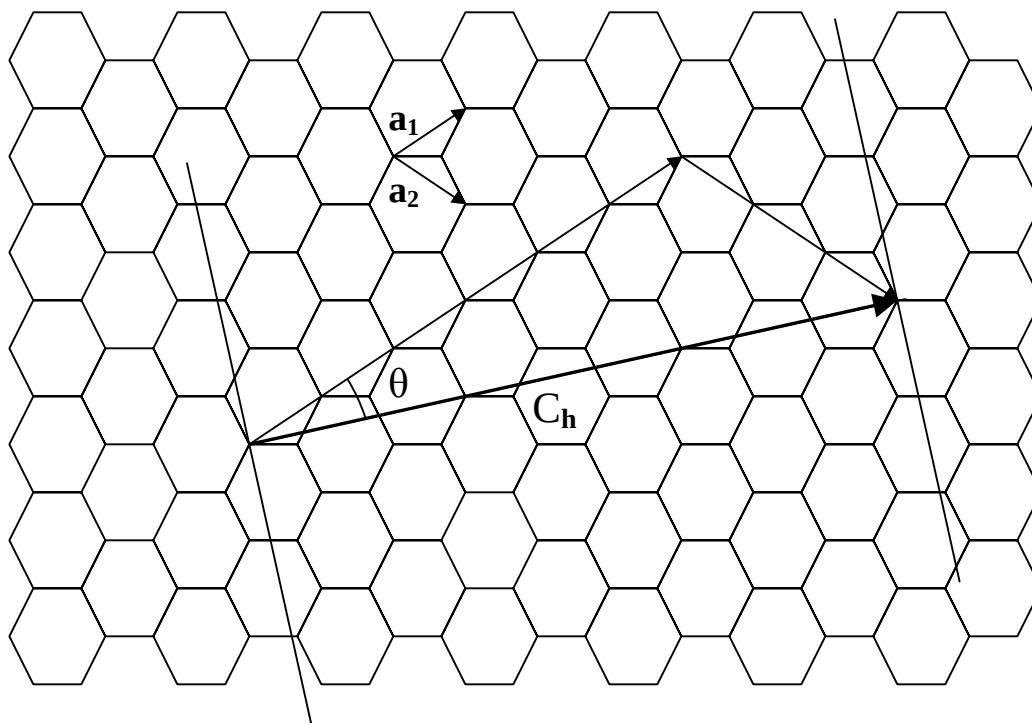
Figure 1. Carbon Nanotube Chiral Vector for a (6, 3) tube
