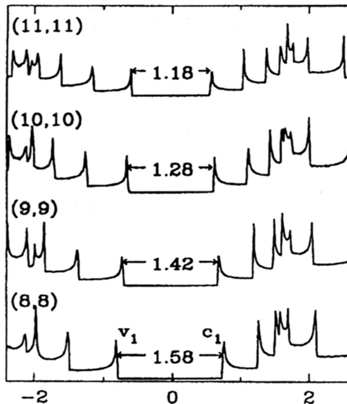
Figure 3. Calculated Electronic DOS Illustrating the Nanotube Size and Band Gap Relationship for a Series of Armchair Nanotubes.
