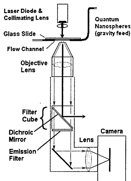
Figure 12. The optical setup: Nikon TE200 inverted microscope with 60X oil-immersion lens, TSI CCD camera, and 35 mW, 405 nm laser diode with collimating lens for illumination.
