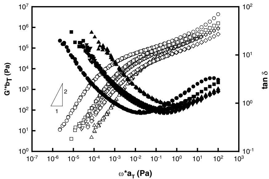
Figure 3. Master Curve of G' (open symbols) and \tan \delta (filled symbols) for as-cast films of iBuPOSS-PS copolymers with varying weight percentage of iBuPOSS: ( \circ ) 0, ( \square ) 6, ( \triangle ) 15, ( \nabla ) 30, and ( \diamond ) 50 wt-% POSS with reference temperature 120 °C.
