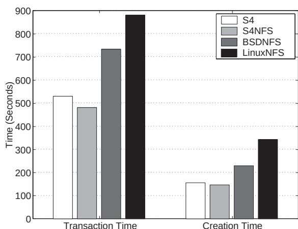
Figure 9-3: PostMark Benchmark Unpack Time (seconds).
