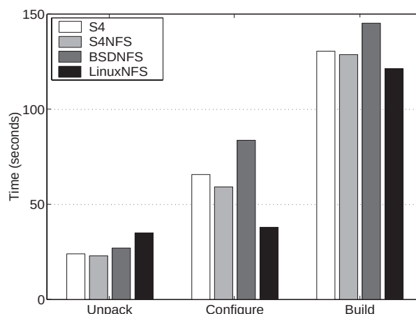
Figure 9-4: SSH-build Benchmark
