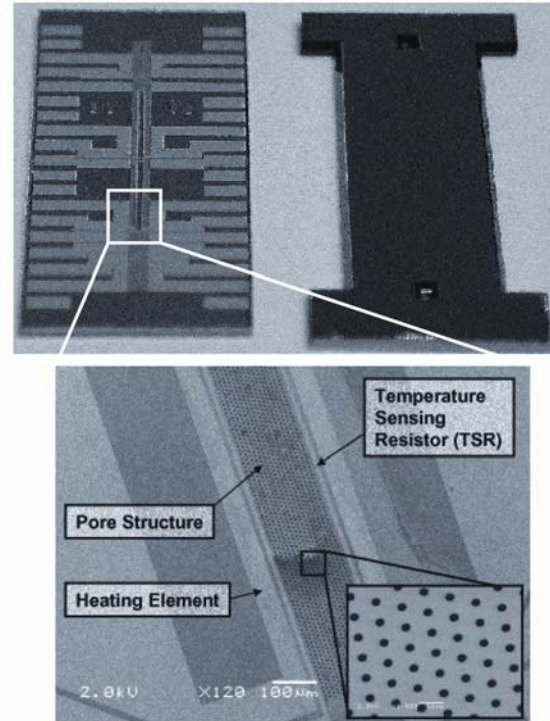
Figure 30: Picture of fabricated microdevice layers prior to packaging, with SEM image of temperature sensing resistor, heating element and membrane pore structure (inset).
