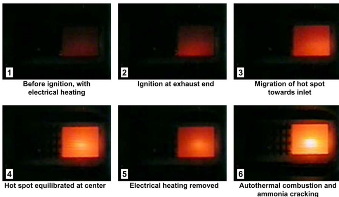
Figure 9. Sequence of images (over the course of \sim 10 s) showing the ignition of a hydrogen in the bottom channel of the reactor, with ammonia flowing in the top channel.
