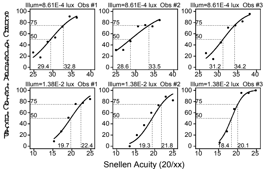
Figure 1. Predicted percent correct adjusted for chance, for each illuminance and observer. Acuity values are given that correspond to 50 and 75% correct adjusted for chance.
