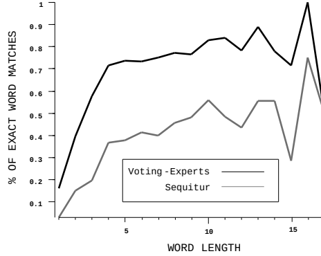
Fig. 2. A comparison of exact match-rate on a per-word basis between SEQUITUR and VOTING-EXPERTS.
